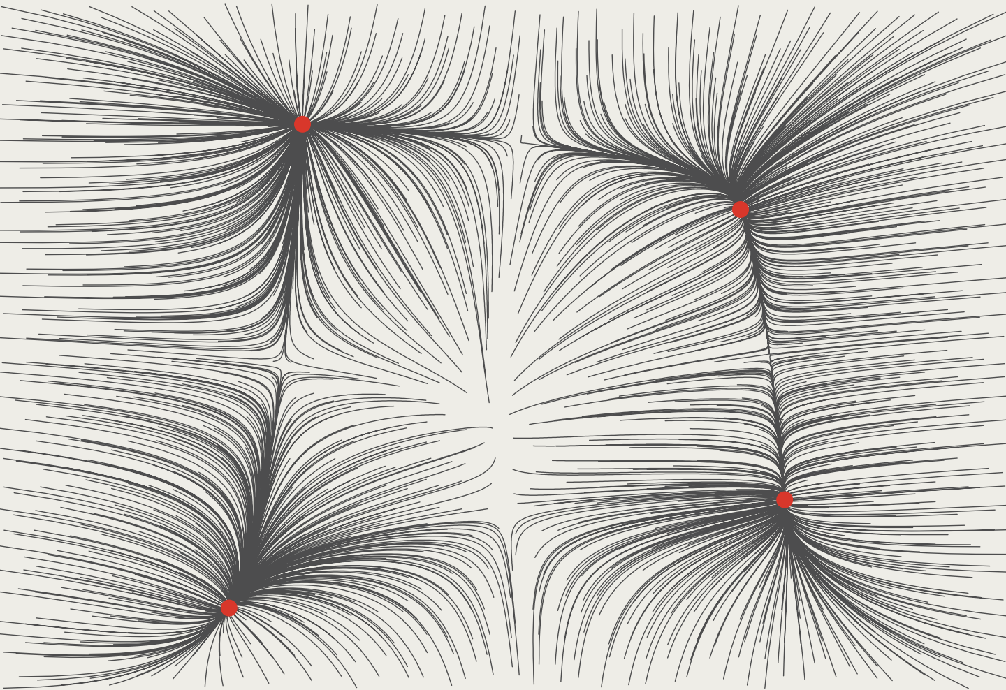
FIG. 0 Gradient descent ( \eta = 0.0006 ) from 1,472 starting points on Himmelblau's function, f(x,y) = (x^2+y-11)^2 + (x+y^2-7)^2 . 503,898 steps in all; every path ends in one of its 4 minima, in red.
