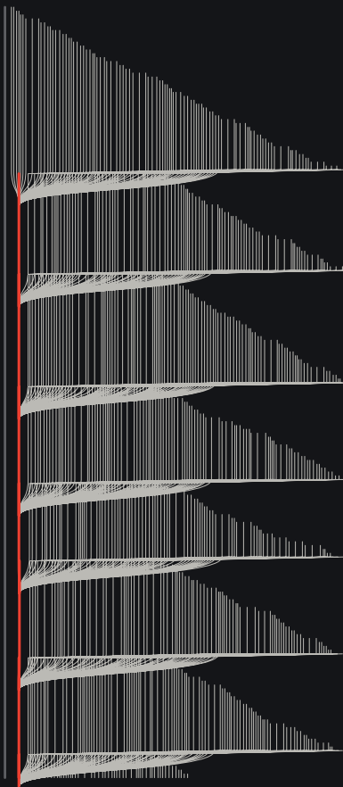
FIG. 0 One simulated 200-turn agent session (464 messages) replayed under three compaction policies. Each line is one message's place in the context window, time running down; where lines converge, the window was compacted (146, 7 and 9 times). Summaries in red.
