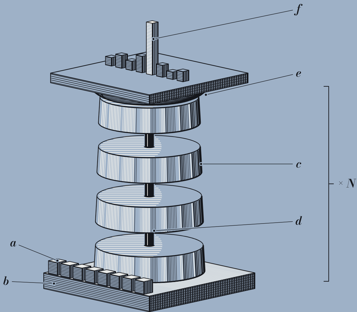
Fig. 1. A decoder-only model, raised as a column. a tokens; b embedding; c a transformer block, one of N ; d the residual stream they are threaded on; e output head; f next-token distribution.
