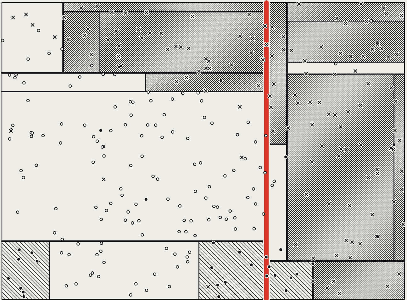
FIG. 0 A classification tree grown in this page by CART – Gini impurity, depth \leq 7 – on 300 labelled points of three classes (rings, dots, crosses). Every line is one question the tree asks, heavier the earlier it is asked; the first is red. 18 questions, 19 leaves, shaded by the class they vote for.
