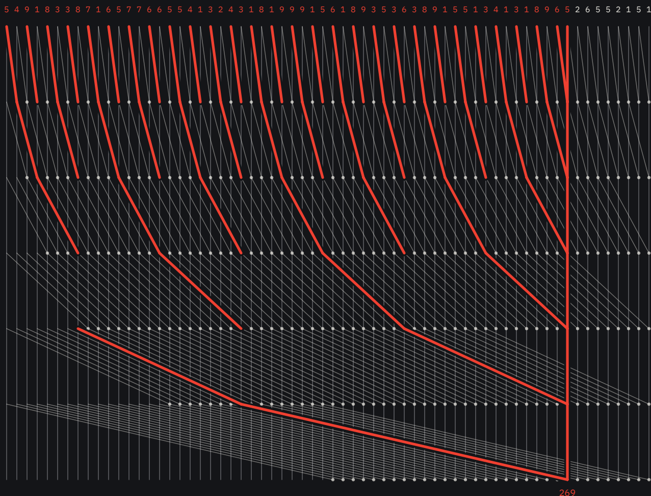
FIG. 0 A Kogge-Stone prefix sum, the pattern inside GPU scan kernels: 64 threads, 6 steps, 321 additions. At step k each thread adds the partial sum 2^k places to its left. In red: the additions thread 55 depends on, gathering 56 of the digits above into 269.
