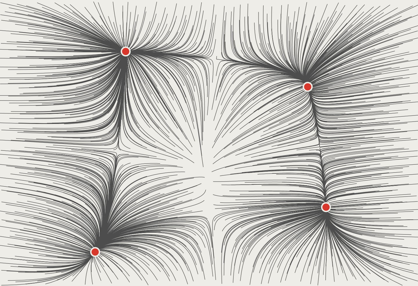
FIG. 0 Gradient descent ( lr = 0.0006 ) from 1,472 starting points on Himmelblau's function, f(x,y) = (x^2+y-11)^2 + (x+y^2-7)^2 . 503,898 steps in all; every path ends in one of its 4 minima, in red.
