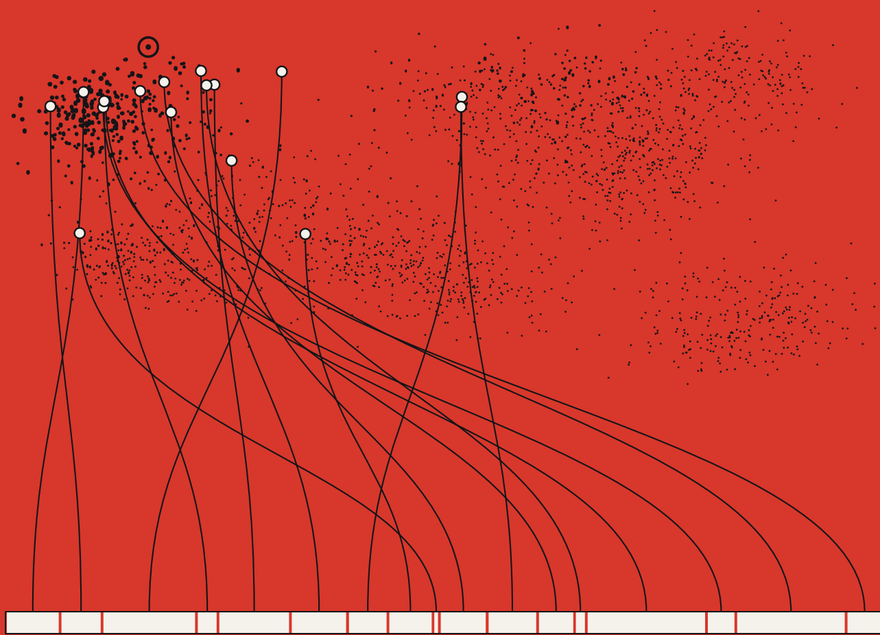
FIG. 0 2,400 synthetic document chunks in a 48-dimensional embedding space, flattened here by PCA; the ringed point is the query. Maximal marginal relevance ( \lambda = 0.55 ) picks the 17 that fill an 8,192-token window (8,190 used), laid out most-relevant-at-the-ends. The chosen are in white.
