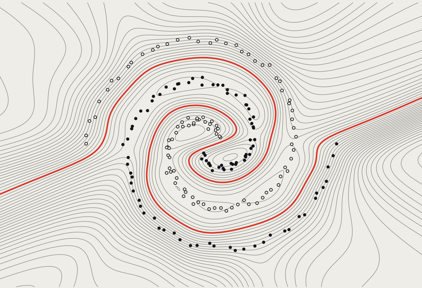
FIG. 0 A 2-16-16-1 tanh network trained in this page – 700 steps of Adam on 192 points of two interleaved spirals. The lines are its output, 47 levels of it; red is the decision boundary it learned (training accuracy 100%).
