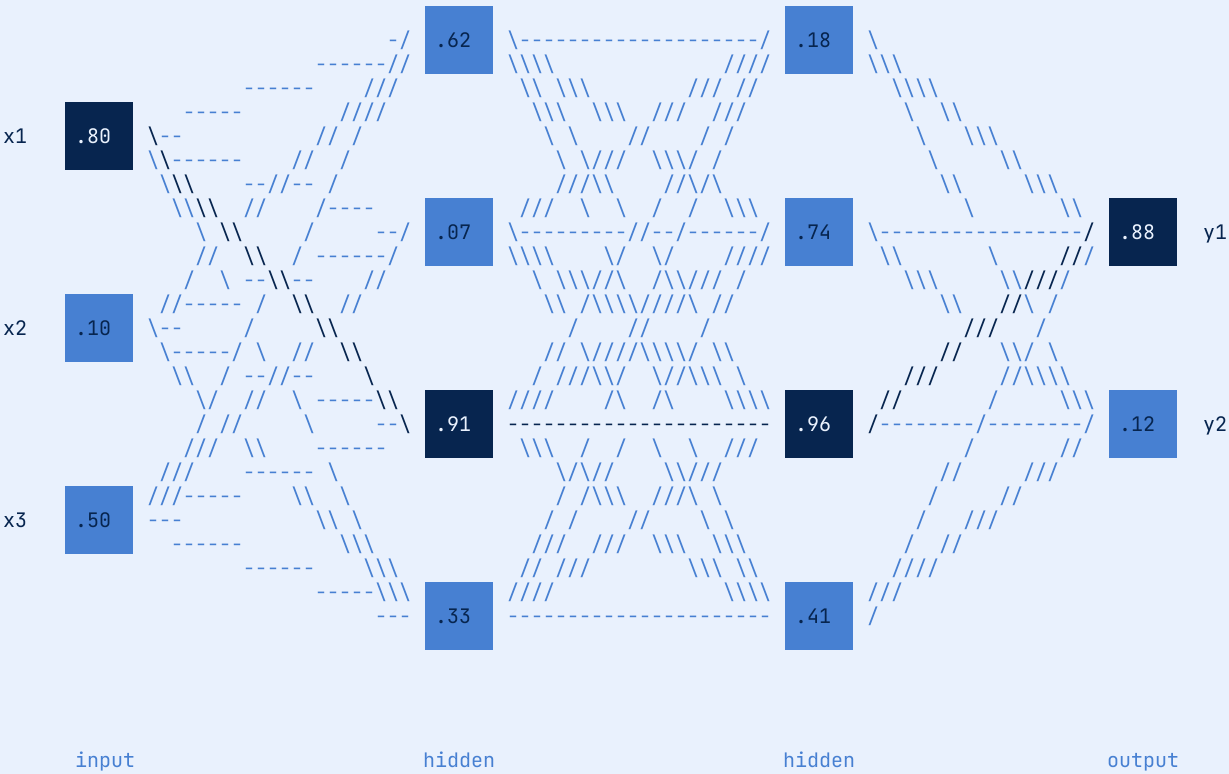
fig. a 3-4-4-2 perceptron, one forward pass lit
