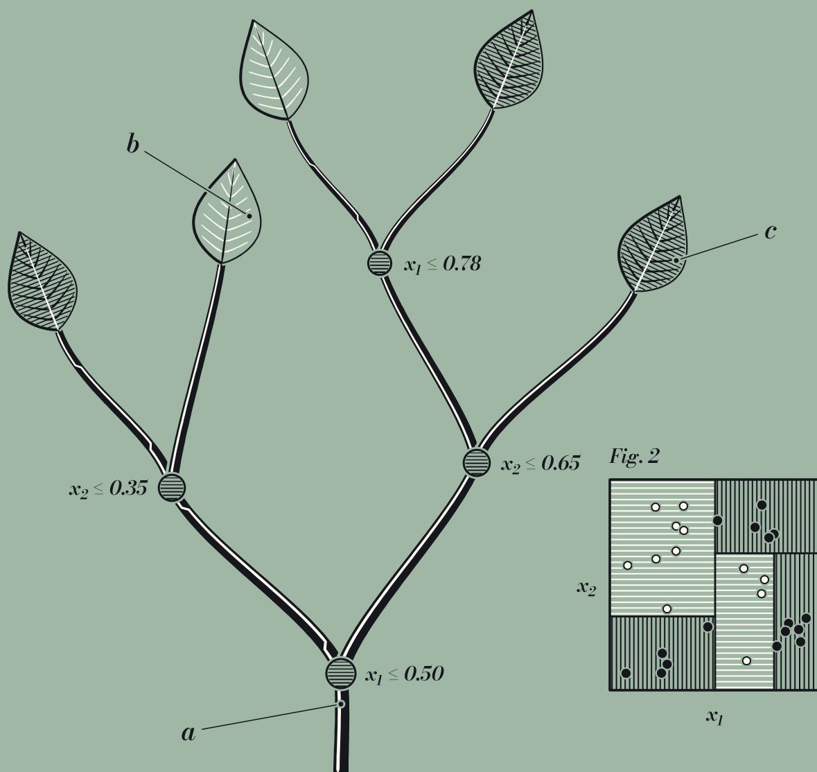
Fig. 1. A decision tree, pressed. a the root split; b a leaf of class A, pale; c a leaf of class B, dark.
