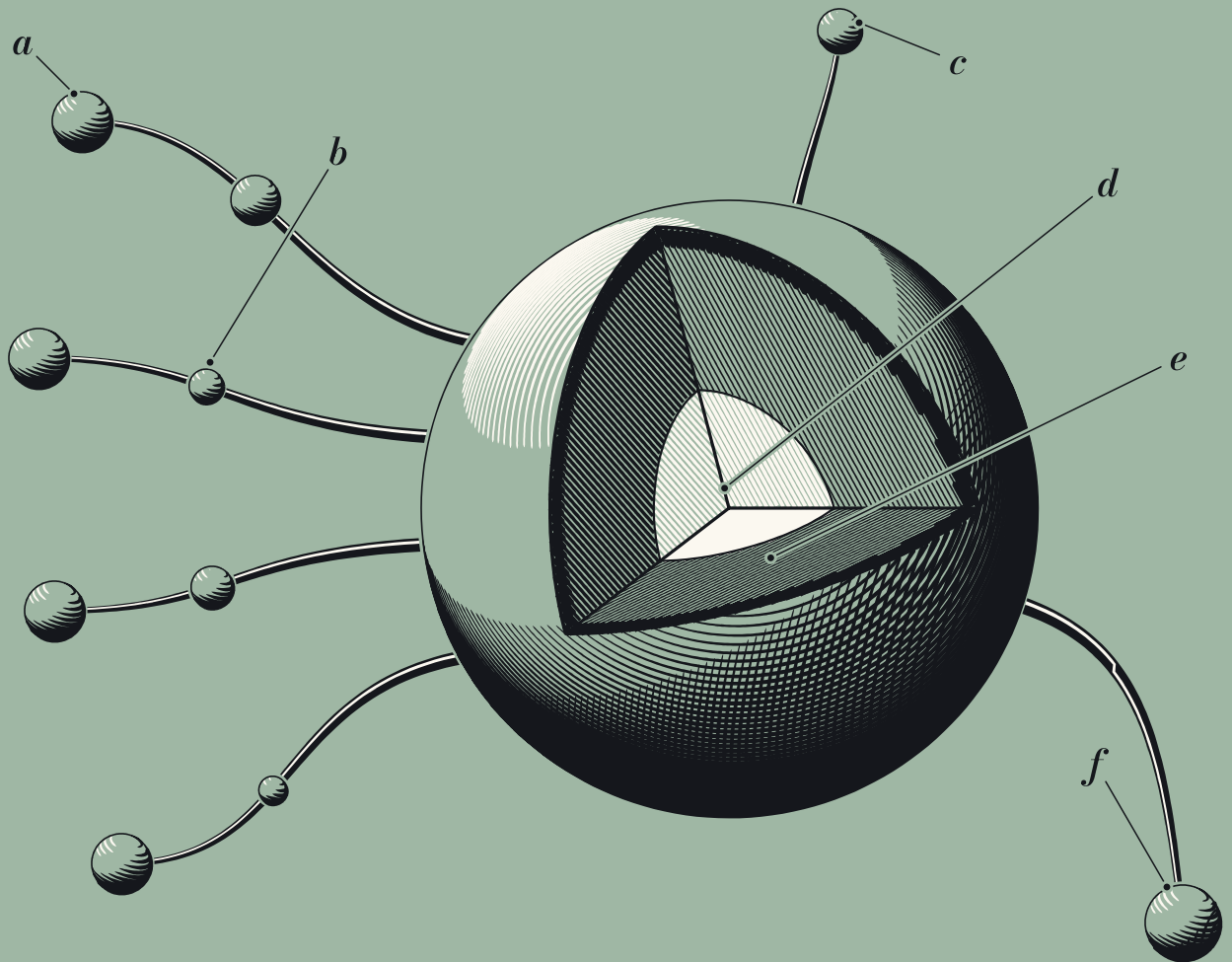
Fig. 1. A single unit, dissected. a inputs; b weights, each bead sized to its magnitude; c bias; d the core, where the weighted sum is formed; e the shell of activation; f output.
