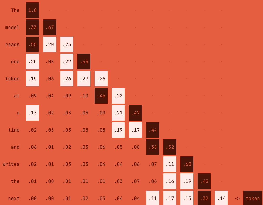
fig. causal self-attention over twelve tokens
