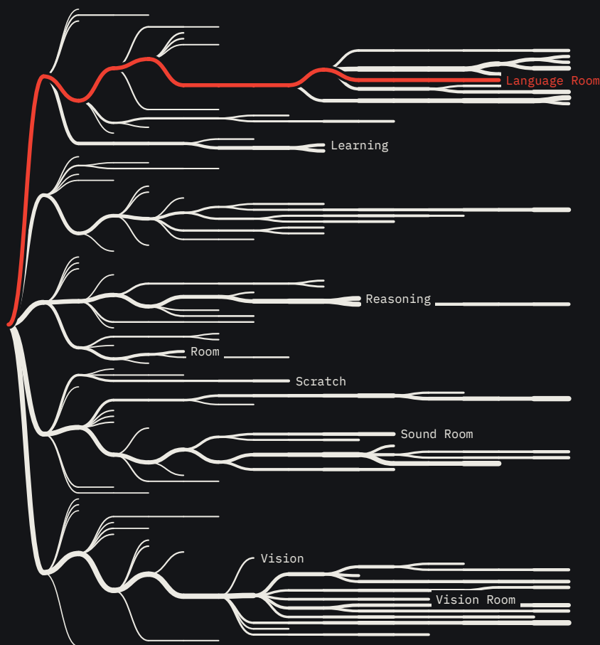
FIG. 0 Beam search (width 32) through a character 5-gram model trained in this page on the 52 titles of this library, continuing “Charlie and the”. Each branch is a letter it weighed, drawn as heavy as it was likely; the labels are titles it finished. In red: this one, its no. 11 guess.
