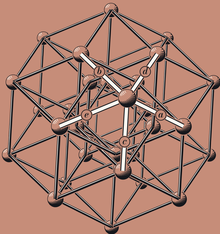
Fig. 1. A device mesh of 2 \times 2 \times 2 \times 2 \times 2 , projected out of five dimensions. From the nearest device, one rod along each axis: a data; b tensor; c pipeline; d sequence; e expert.
