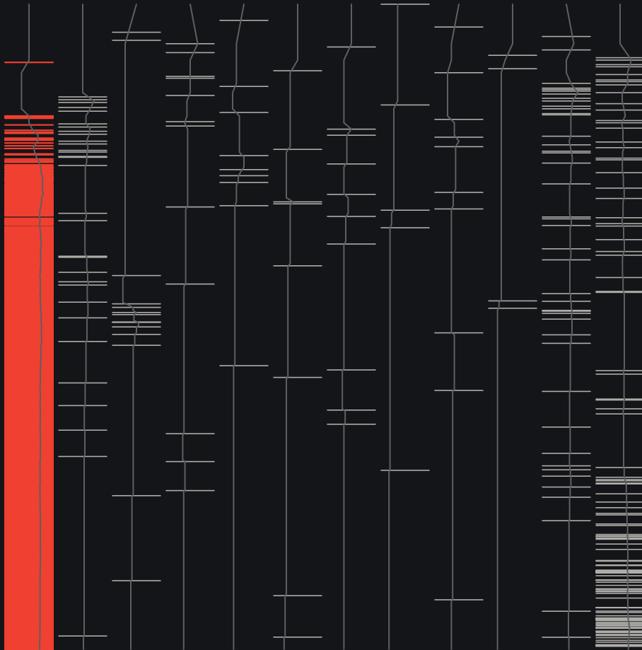
FIG. 0 Thompson sampling on a 12-armed bandit, 1,600 pulls computed in this page, time running down (on a square-root scale). Each dash is one pull; the thin line in each column is the agent's belief about that arm. The best arm ( p = 0.72 ) is red: it was pulled 1,345 times of the 1,600 and paid out 990.
