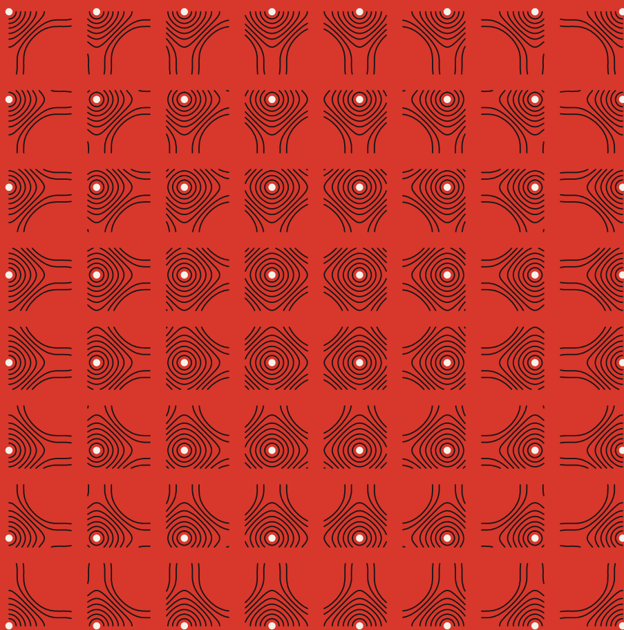
FIG. 0 A Vision Transformer reads a picture as an 8 \times 8 grid of patches and tells them apart by position embeddings – here the fixed 2-D sine-cosine kind used by MAE and Simple ViT ( d = 256 ). Each small field contours one patch's cosine similarity to every position; white marks the patch itself.
