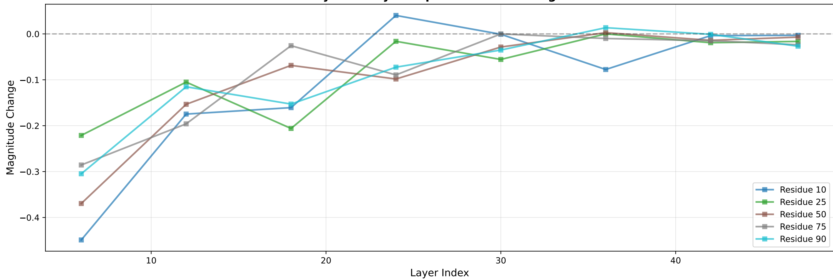
Layer-to-Layer Representation Changes
