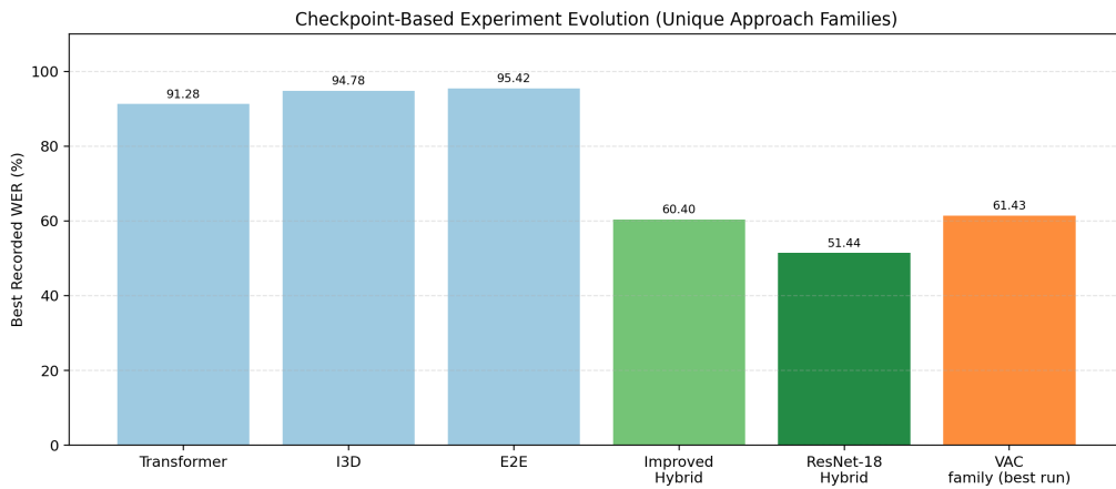
Figure 5.1: Checkpoint-based experiment evolution in terms of best recorded WER.
