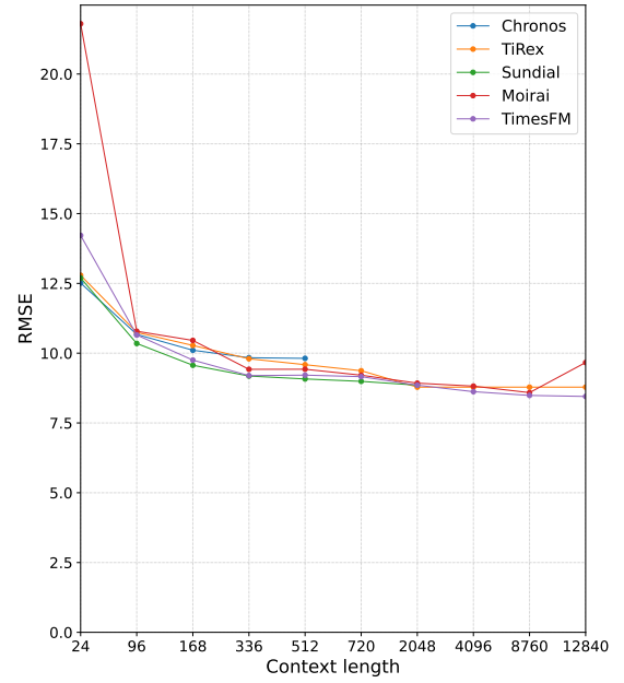
(b) RMSE for different context lengths
