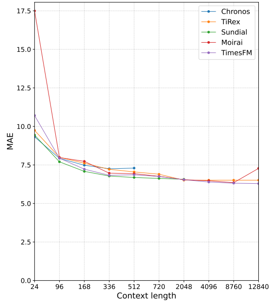
(a) MAE for different context lengths
