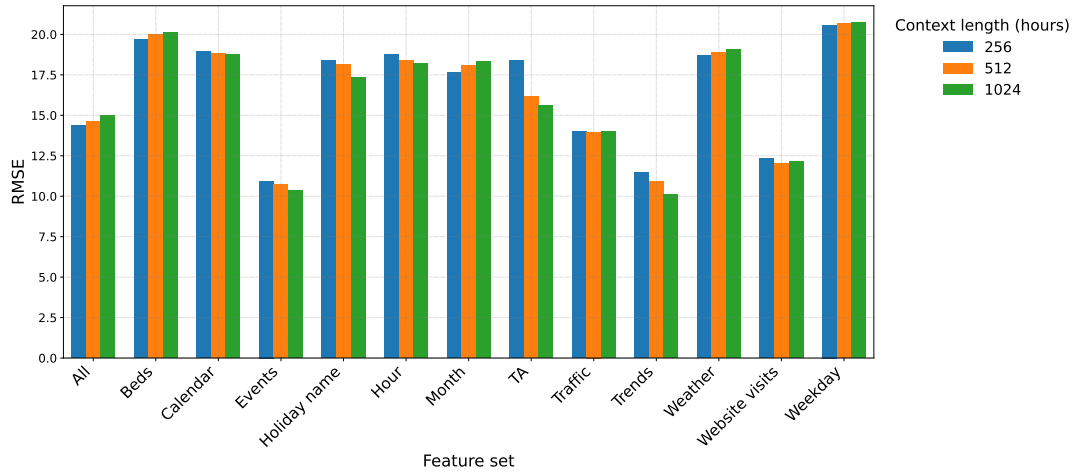
(b) RMSE for different subsets
