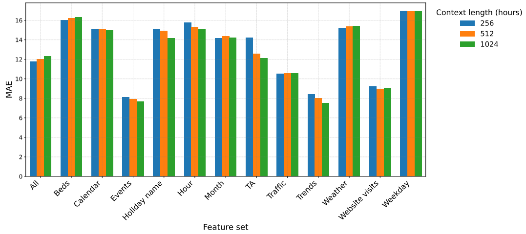
(a) MAE for different subsets
