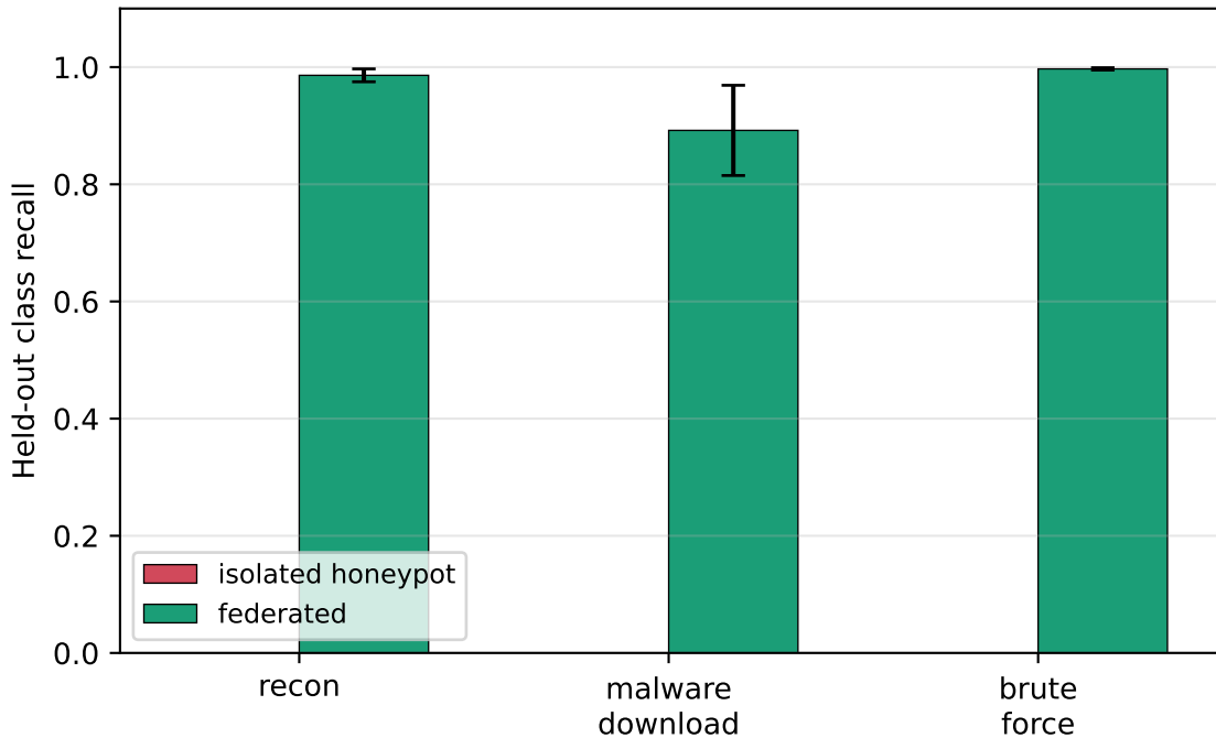
Isolation fails; federation recovers (honeypots)
