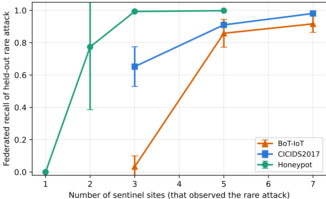
Sentinel threshold generalizes across data types
