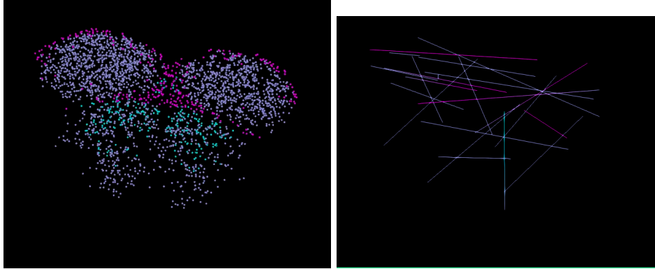
Figure 21: Isolated Coma Connectome, showing 2800 nodes (out of 28662) and key pathways, contributing to onset of Coma (Mid Brain)
