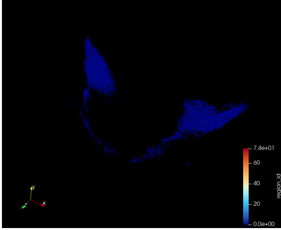
(a) PAL (pallidum) voxels alone. PAL is spatially distributed across the connectome – it forms a hub with projections to multiple core regions, creating a new H_1 cycle and raising b_1 : 1 \rightarrow 2 .
