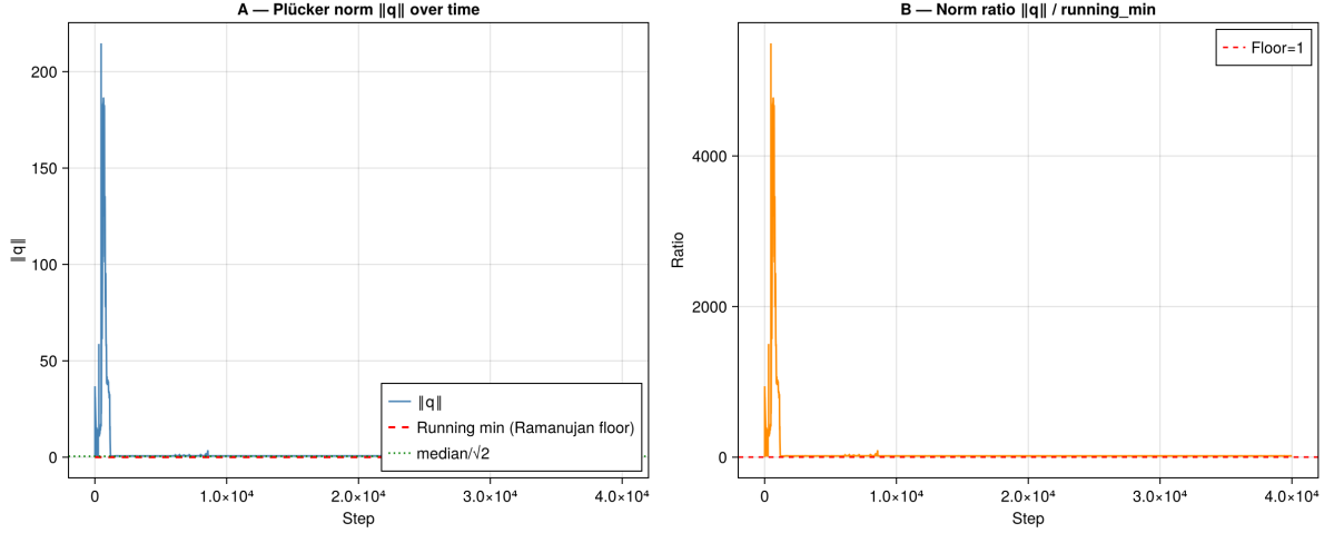
Figure 18: A : Plücker norm \|q\| over the full simulation ( \approx 40,000 steps). The initial spike to \|q\| \approx 215 corresponds to the sAMY curvature driving the bicharacteristic far from \text{Gr}(2, 4) ( K_{\text{max}} = 3.85 ): the surface \Sigma_Q develops deep orbifold structure. Exponential decay to \|q\| \approx 0 (the Klein quadric) with Lyapunov rate \lambda \approx -0.104 : the bicharacteristic returns to the characteristic variety \Lambda_{\text{red}} [KS94]. B : Norm ratio \|q\| / \|q\|_{\min} . The ratio reaches \approx 4500 at peak and decays to 1.0 by step \approx 10,000 , confirming that the bicharacteristic completes its excursion and returns to the Klein quadric — the sphere limit of Remark A.10.
