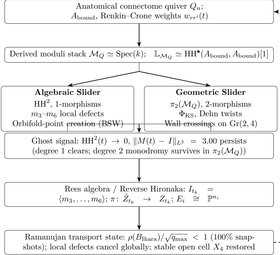
Figure 10: The derived (2, 1) -stack \mathcal{M}_Q as the unifying canvas. Each node is a coordinate chart on \mathcal{M}_Q ; arrows show the logical flow from connectome data to observed phenomena. The dashed feedback arrow is the simulation loop: Rees-resolved state feeds back as new weights w_{rr'}(t+1) .
