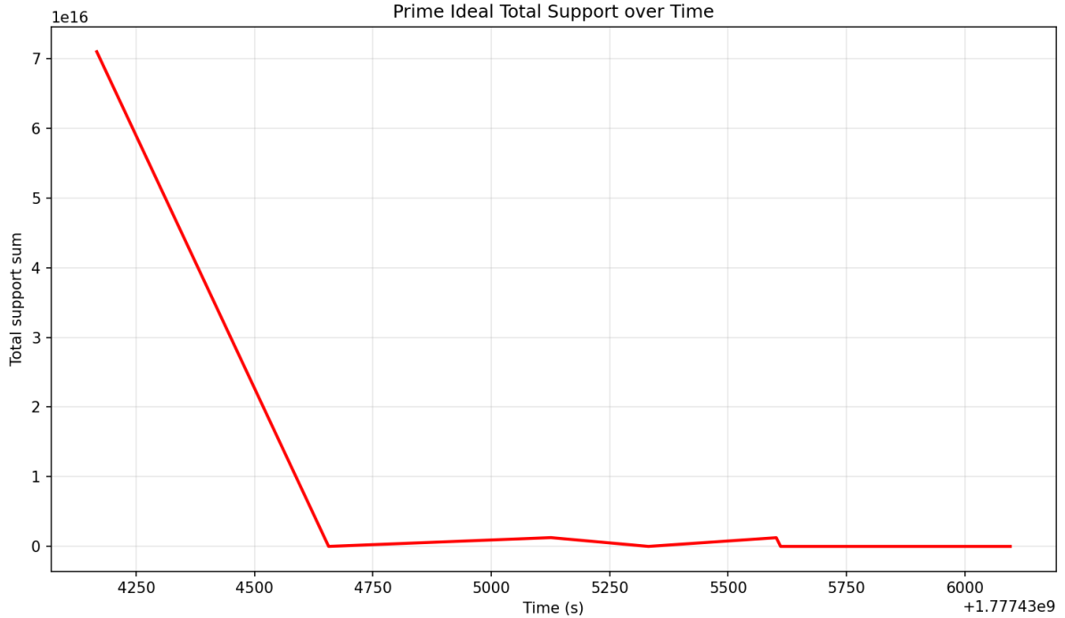
Figure 4: Prime ideal total support over time: evidence for the continuation functor \rho_{ij} . The total support \sum_{p \in I_\tau} \|p\| of the active prime path ideal decays from 7 \times 10^{16} to \approx 0 within \sim 400 s of the wall-crossing event (snapshot \sim 4600 s), then remains near zero. This is the experimental signature of the admissible continuation functor \rho_{0,3} : \mathcal{A}_0(\mathcal{F}) \rightarrow \mathcal{A}_3(\mathcal{F}') (Definition 5.3): the prime ideal basis I_{\tau_1} of sector k = 0 is replaced by I_{\tau_2} of sector k = 3 as the bicharacteristic crosses \Lambda_{\text{red}}^+ in the forward direction. By Theorem 5.4(iii) (Ihara invariance), the Ihara H_1 eigenvalues \{1.7898, -0.8021\} remain constant throughout this transition the continuation functor preserves the Ihara spectrum while redistributing the local prime ideal support.
