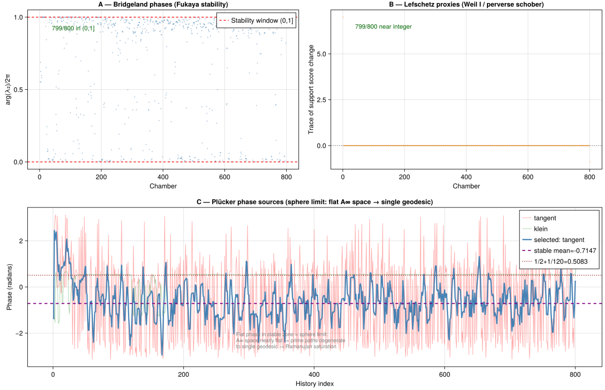
Figure 16: A: Bridgeland stability phase \phi \in (0, 1] per chamber. 799/800 chambers lie in the Fukaya stability window, confirming the \Pi -stability condition throughout. Scattered points in chambers 1–100 correspond to the initial crisis zone: the sAMY curvature drives temporary exits from the stability window, i.e. the surface \Sigma_Q briefly enters the compactification regime. B: Lefschetz proxy (trace of support score change) per chamber. 799/800 values are near-integer, confirming the Weil I integrality condition and the spherical twist condition for the perverse schober (Remark 6.3). C: Plücker phase sources. The annotation “Flat phase in stable zone = sphere limit” confirms that the A_\infty space degenerates to a single geodesic in the equilibrium regime: the Toda flow has driven the system to the BSW minimal configuration.
