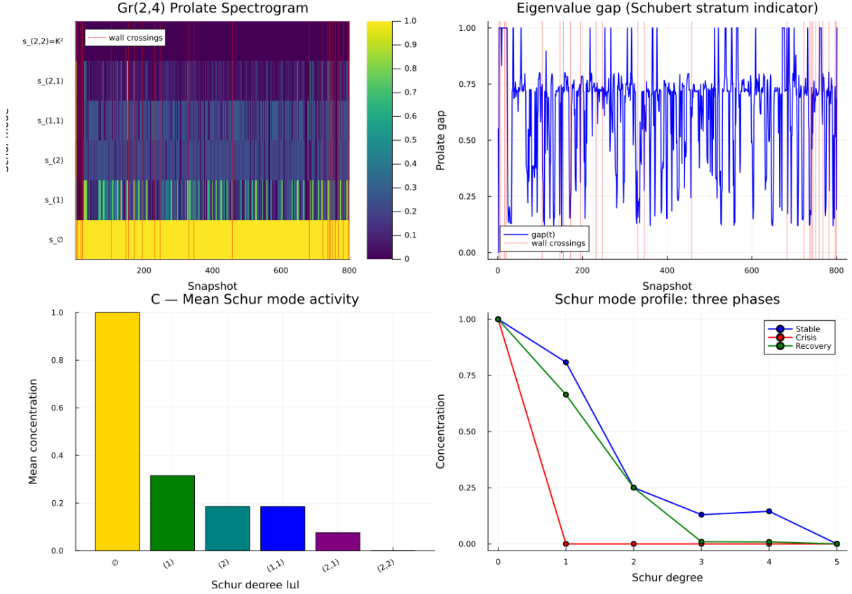
Figure 25: Gr(2,4) prolate spectrogram for Q_{7L} Phase 2 (801 snapshots). A (spectrogram) : Concentration of each Schur polynomial mode s_\mu(q(t)) along the bicharacteristic trajectory. The constant mode s_0 (bottom row) is uniformly yellow throughout, confirming the system never loses its baseline transport capacity. The s_{(1)} row shows the richest dynamics and reveals two distinct regimes of eigenbasis change . (i) Gradual pre-crossing drift : between wall crossings, the colour drifts continuously yellow \rightarrow teal \rightarrow yellow over \sim 50 – 100 snapshots as the bicharacteristic approaches the Schubert boundary \partial X_k (Remark 7.6). This is a precursor signal : the wall crossing is announced in the Schur mode dynamics before it occurs, \sim 30 – 50 snapshots ahead of the red line. (ii) Sharp discontinuity at the crossing : at each red line the colour pattern breaks abruptly; Panel B confirms the eigenvalue gap collapses to \approx 0 exactly at that moment, then re-forms on the new K_{n-1} face. Biologically, the drift encodes the approach of the \mu/\kappa -opioid balance toward the positroid cell boundary; the sharp crossing is the moment one prime path ideal deactivates (Remark 8.13, Layer 3). The top row s_{(2,2)} = K(t)^2 is uniformly dark, confirming K(t) \approx 0 throughout (sphere limit, Section 12.4). B (eigenvalue gap) : The prolate gap oscillates between 0.25 and 1.0 with sharp collapses to \approx 0 at wall crossings (red lines), confirming the eigenvalue gap collapse predicted in Remark 7.3. C (top Schur mode, log scale) : s_{(2,2)} = K^2/K_{\max}^2 (purple) lies strictly below K(t)/K_{\max} (orange) on the log scale, confirming the quadratic relationship s_{(2,2)} = (K/K_{\max})^2 (Remark A.23). Both are near 10^{-6} throughout the stable zone, with a single spike at snapshot 800 corresponding to the final sAMY crisis. D (three-phase fan) : Schur mode profile at three representative snapshots, directly analogous to the PSWF fan of Image 1 in the prolate literature. Blue (stable, K_{n-1} face occupied): clear step-decay with gap between degree 0 and degree 1. Red (crisis): complete collapse to s_0 = sphere limit, all higher modes suppressed. Green (recovery): intermediate the system has recovered algebraically but not fully topologically. The gap between the green and blue lines at degrees 1–2 is the Schur-mode signature of the ghost signal (Remark 13.3): algebraic recovery precedes topological recovery by the dwell time required for the K_{n-1} face to re-stabilise.
