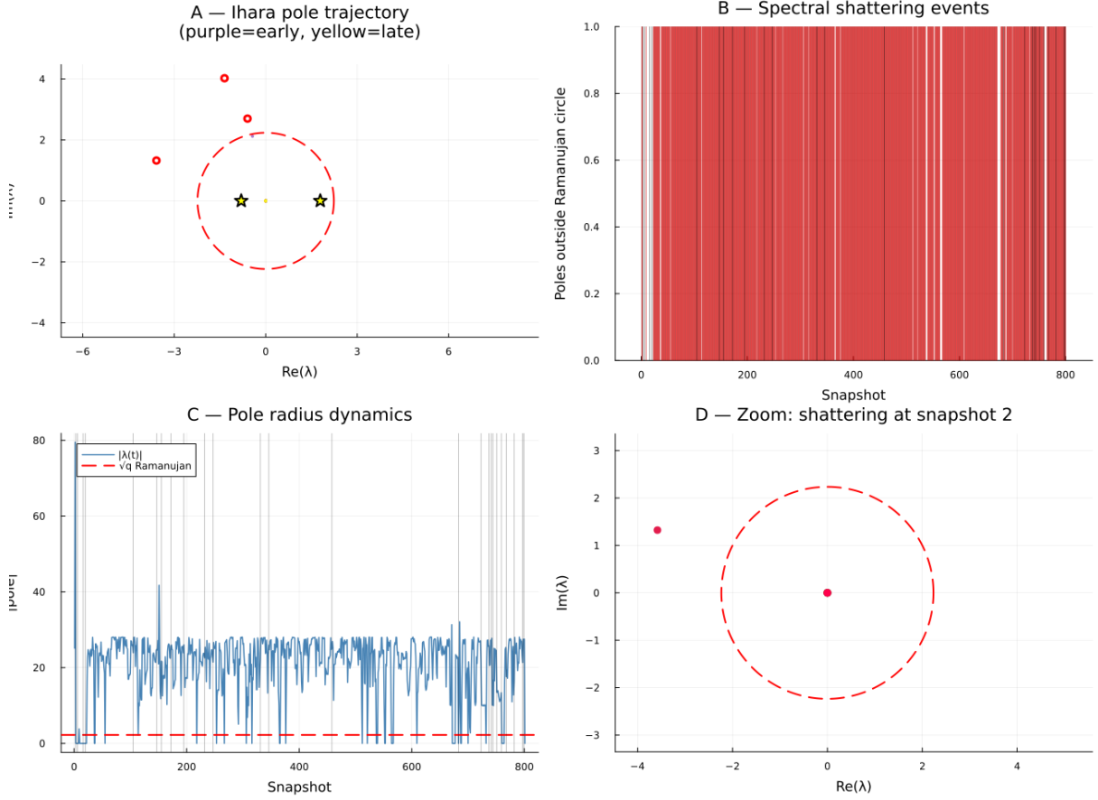
Figure 26: Ihara pole dynamics for Q_{7L} Phase 2. The dynamic poles plotted are the eigenvalues of the complex spectral gap \lambda(t) = \text{gap\_re}(t) + i \cdot \text{gap\_im}(t) , the time-varying eigenvalue of the effective transport operator at each snapshot. The red dashed circle is the Ramanujan bound |\lambda| = \sqrt{q_{\max}} \approx 2.236 . Gold stars mark the fixed H_1 eigenvalues \lambda_1 = 1.7898 and \lambda_2 = -0.8021 of B_{\text{Ihara}} (MAGMA exact, time-independent). A (pole trajectory): Three stray poles (white-ringed red circles) are visible outside the Ramanujan circle, at positions \approx (-3.5, 1.1) , (-2.5, 2.9) , and (-2.0, 3.8) . These correspond to the early-snapshot crisis zone (purple, snapshots 1–30) where the m_0 = 5.0 curvature drives the bicharacteristic far from \Lambda_{\text{red}} . B (shattering count): The dynamic gap eigenvalue exceeds \sqrt{q} for the majority of snapshots, reflecting that the raw transport amplitude |\lambda(t)| is not the same as the MAGMA-exact \rho(B_{\text{Ihara}})/\sqrt{q} = 0.7865 < 1 (the Ramanujan bound applies to B_{\text{Ihara}} , not to the dynamic gap eigenvalue; Remark 8.13, Layer 2). C (pole radius): The radius oscillates 0–80 with large spikes at wall crossings (grey lines). The floor near the Ramanujan circle (red dashes) during the sphere-limit phase ( K(t) \approx 0 ) confirms that the dynamic eigenvalue converges toward B_{\text{Ihara}} ’s fixed spectrum as the system stabilises. D (zoom, snapshot 2): One pole inside the circle ( \approx (0, 0) ) and one outside ( \approx (-3.8, 1.3) ) at the first shattering event. The inside pole is the stable H_1 mode; the outside pole is the transient crisis mode generated by the m_0 curvature before the bicharacteristic has re-entered \Lambda_{\text{red}} .
