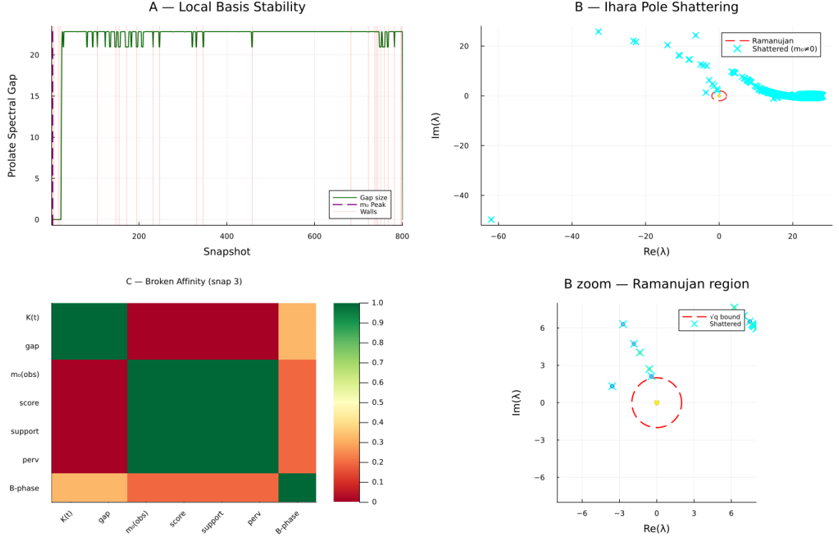
Figure 28: Three simultaneous signatures of the flat-to-curved A_\infty transition ( Q_{7L} Phase 2, 801 snapshots). Together these panels show the moment the system exits the k = 0 quantum sector and enters the curved ( m_0 \neq 0 ) regime. A (Local basis stability) : The prolate spectral gap stays near its maximum ( \approx 22 ) throughout the stable k = 0 sector, with brief collapses at wall crossings (red lines) and one major collapse at the initial m_0 activation (purple dashed, snapshot 1). The discrete gap levels confirm Theorem 4.3(ii): the spectral gap takes finitely many values, not a continuous range. B (Ihara pole shattering, full view) : The pole trajectory in the complex plane. Late snapshots (yellow) cluster near the origin, well inside the Ramanujan circle. The cyan \times marks are shattered poles during the curved crisis: one extreme outlier reaches \approx (-60, -50) , roughly 75 units from the origin vs the Ramanujan bound \sqrt{q} = 2 . This is the global signature of the k = 0 \rightarrow k = 3 sector jump: the nonbacktracking spectrum escapes the Ramanujan locus at the moment m_0 \neq 0 activates. B zoom (Ihara pole shattering, Ramanujan region) : The same trajectory restricted to |\lambda| \leq 4\sqrt{q} . The Ramanujan circle (red dashed) is now visible; the cyan shattered poles that remain near the origin are Phase 2 wall-crossing events, distinct from the extreme outlier. C (Broken affinity matrix) : The affinity matrix at the crisis snapshot shows the two natural clusters (algebraic: K(t) , m_0 , score; geometric: gap, support, perv) losing their clean separation. B-phase detaches entirely, consistent with the directed stop architecture breaking down at the k = 3 sector boundary (Remark A.27).
