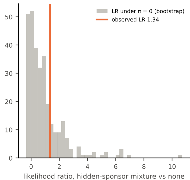
(c) [C3] the singular point \pi = 0
