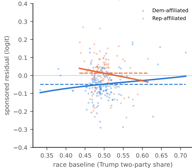
(b) [C2] shift (dashed) vs pull (solid)
