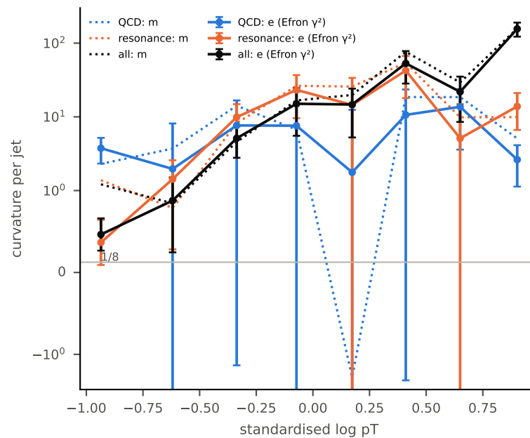
(e) where flat transport fails, all jets (1e-3 nats/jet) excess 0.12 \pm 0.06 , z 2.0
