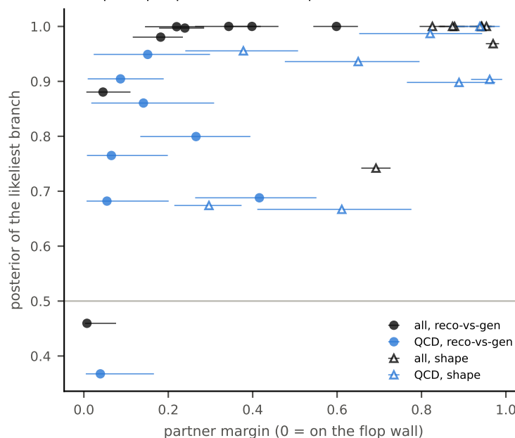
(h) branch certainty is set by distance to the wall (one point per pT bin; bars 90% posterior)
