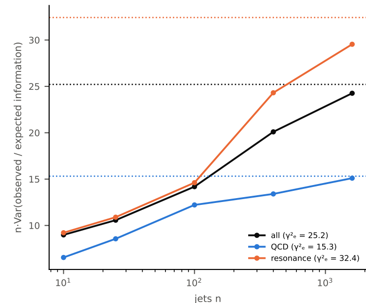
(c) curvature = how much the error bar wobbles (dotted: Efron-Hinkley prediction \gamma^2_e )
