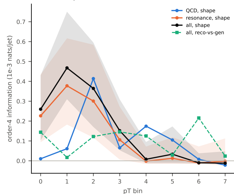
(i) information only the 4-way joint carries (bands 90% posterior; QCD band omitted: \pm 0.5 )
