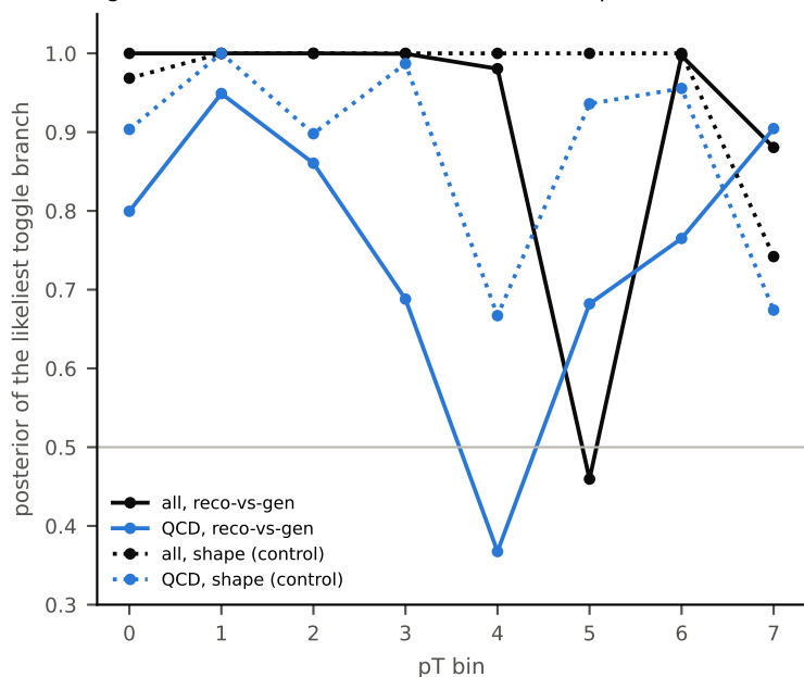
(g) near a node the branch is uncertain (flop)
