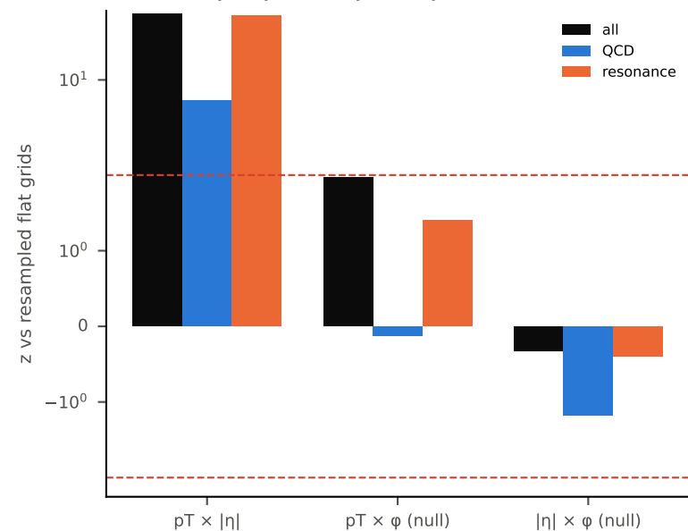
(f) holonomy only where symmetry allows it
