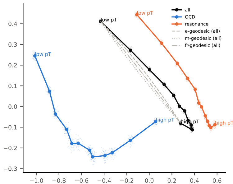
(a) pT paths on the Fisher sphere x = 2\sqrt{p} (PCA, 93% of spread; clouds = posteriors)
