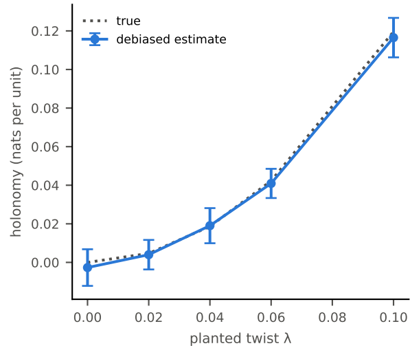
(b) holonomy 2-form: flat \rightarrow 0
