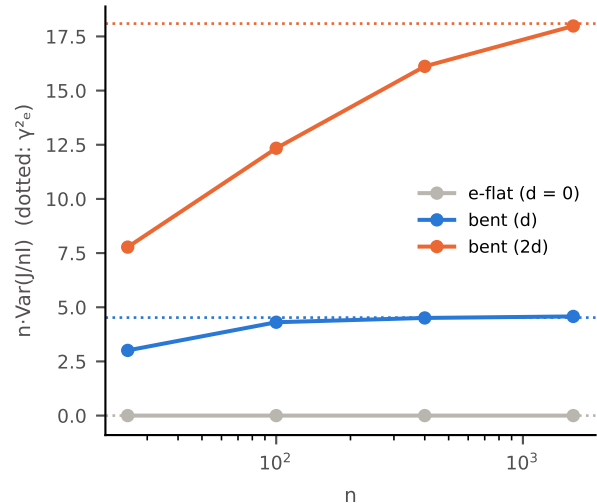
(c) curvature = information wobble
