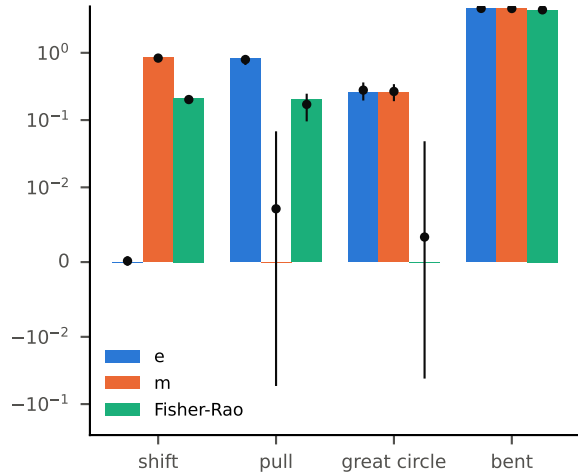
(a) each geodesic has zero curvature in its own connection (dots: estimated)
