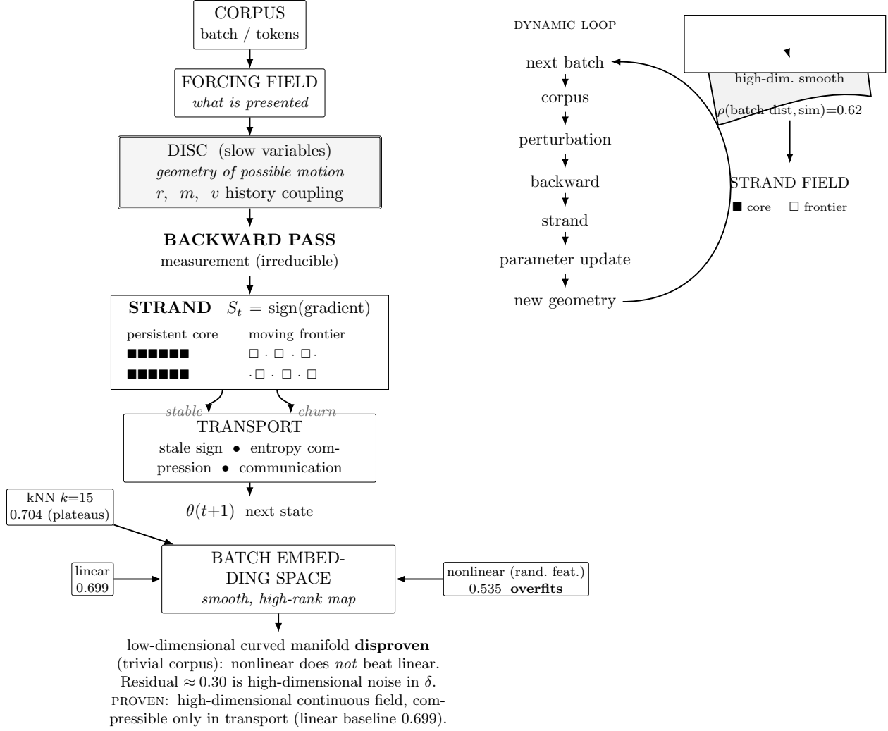
FIGURE 7. The disc-strand picture as measured. Left: the pipeline — a smooth, high-dimensional corpus forcing field selects the strand’s identity (not its magnitude); the disc (r, m, v) is the slow manifold (geometry of possible motion, not a controller: it sets persistence and the fixed \sim 55\% /step churn velocity but cannot generate or gate the strand); the irreducible backward pass produces S_t = \text{sign}(g_t) , split into a persistent core ( \sim 115\text{k} coordinates) and a frontier sweeping 99.6\% of the network; only transport downstream compresses (stale-sign, 79\times sign entropy). Middle: the training loop — corpus perturbation, measurement, strand, update, new geometry. Right: the disc as a high-dimensional smooth manifold; nearby batches give nearby strands (batch-distance/similarity \rho=0.62 ), strand fields orbiting it with the core/frontier split. Bottom: the batch \rightarrow strand map is smooth but high-rank — linear predicts strand sign at 0.699, kNN plateaus at 0.704, and a nonlinear model fails to beat linear (0.535, overfits), disproving a low-dimensional curved manifold for this corpus. The corpus signal is real and continuous but high-dimensional, with a \approx 0.30 residual living in the backward error \delta ; whether a structured corpus yields a low-dimensional map is the one open question (§41.11).
