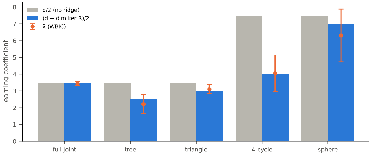
The ridge lowers \lambda by \dim \ker R / 2
