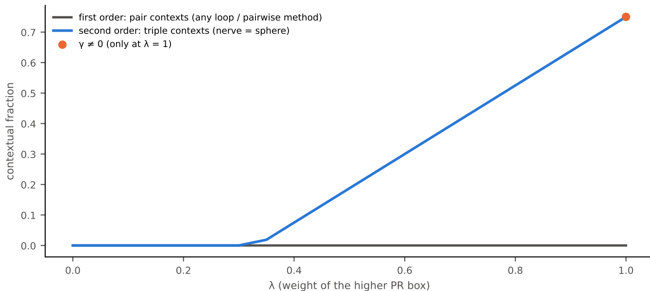
(d) the obstruction is invisible to first-order (pairwise) views
