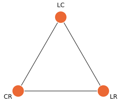
(a) triangle cover, contradictory pairs: hollow Betti (1, 1); graph loops 1, filled 0; CF 1.00
