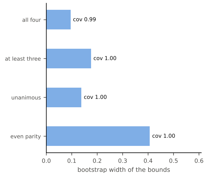
(e) MBIC 4-group outcomes: width, coverage
