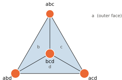
(b) tetrahedral cover, higher PR box Betti (1, 0, 1); graph loops 3, filled 3; CF 0.75
