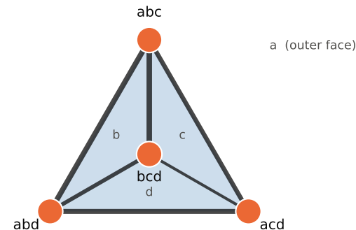
(c) tetrahedral cover, MBIC (one split) Betti (1, 0, 1); graph loops 3, filled 3; CF 0.15
