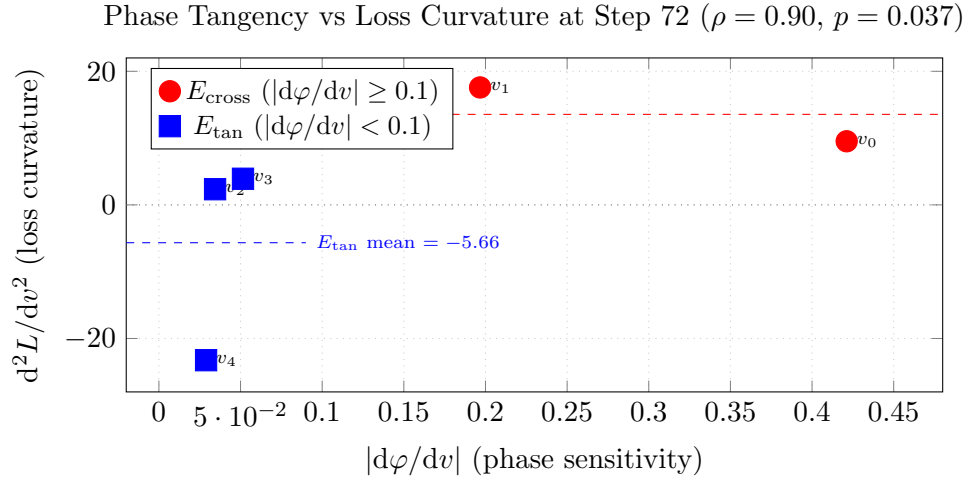
FIGURE 4. Phase sensitivity |d\varphi/dv| vs loss Hessian curvature d^2L/dv^2 for the five null eigenvectors at step 72 (Spearman \rho = 0.90, p = 0.037, n = 5 ). Red circles ( E_{\text{cross}}, v_0 and v_1 ): large phase sensitivity, positive loss curvature (loss-ascent directions). Blue squares ( E_{\text{tan}}, v_2, v_3, v_4 ): small phase sensitivity, negative or small loss curvature (loss-descent or flat directions). The phase-tangent directions at the codimension-2 crossing are precisely the loss-descent directions in the symplectic null space.
