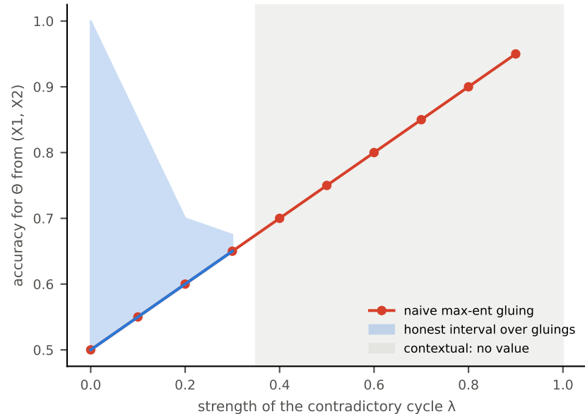
(c) across an obstruction the value is an interval, then undefined
