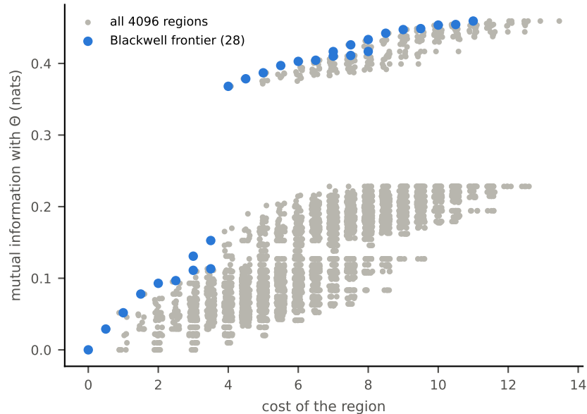
(a) reward-free pruning ( n = 12 ): every optimum lies on the frontier (147/147 cases)
