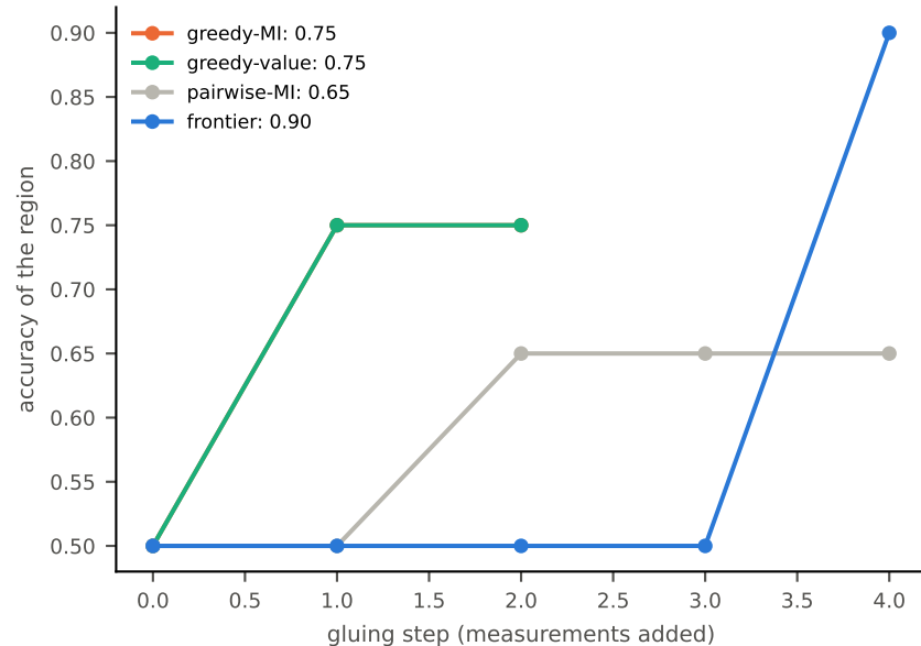
(b) the parity path is flat until its last step: invisible to pairwise and myopic grading
