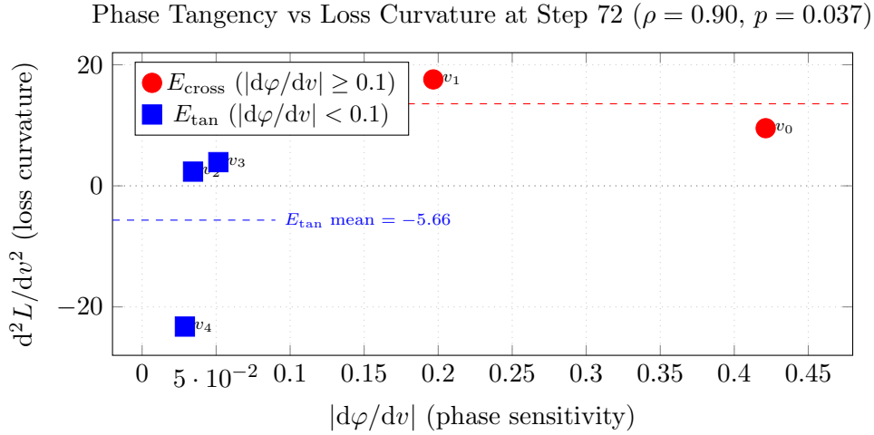
FIGURE 4. Phase sensitivity |d\varphi/dv| vs loss Hessian curvature d^2L/dv^2 for the five null eigenvectors at step 72 (Spearman \rho = 0.90 , p = 0.037 , n = 5 ). Red circles ( E_{\text{cross}} , v_0 and v_1 ): large phase sensitivity, positive loss curvature (loss-ascent directions). Blue squares ( E_{\text{tan}} , v_2, v_3, v_4 ): small phase sensitivity, negative or small loss curvature (loss-descent or flat directions). The phase-tangent directions at the codimension-2 crossing are precisely the loss-descent directions in the symplectic null space.
