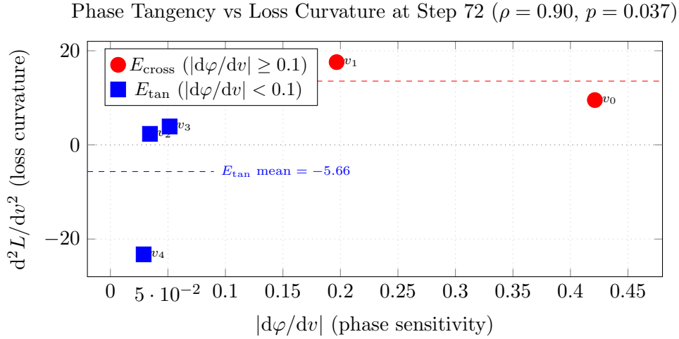
FIGURE 3. Phase sensitivity |d\varphi/dv| vs loss Hessian curvature d^2L/dv^2 for the five null eigenvectors at step 72 (Spearman \rho = 0.90 , p = 0.037 , n = 5 ). Red circles ( E_{\text{cross}} , v_0 and v_1 ): large phase sensitivity, positive loss curvature (loss-ascent directions). Blue squares ( E_{\text{tan}} , v_2, v_3, v_4 ): small phase sensitivity, negative or small loss curvature (loss-descent or flat directions). The phase-tangent directions at the codimension-2 crossing are precisely the loss-descent directions in the symplectic null space.
