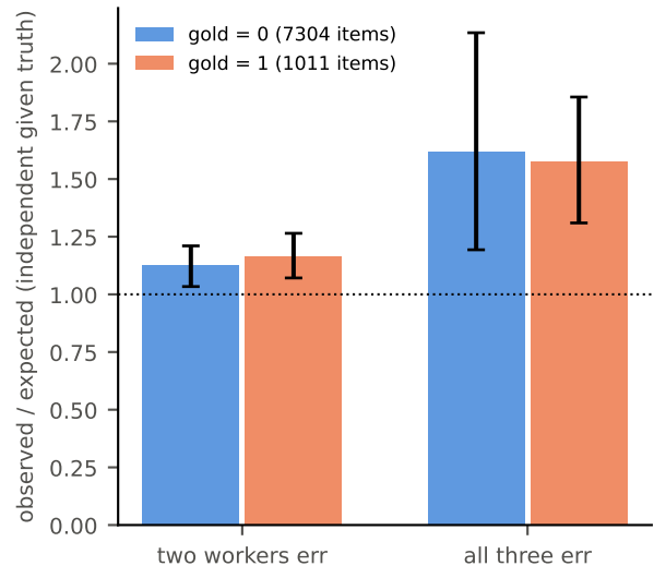
(b) co-errors exceed conditional independence
