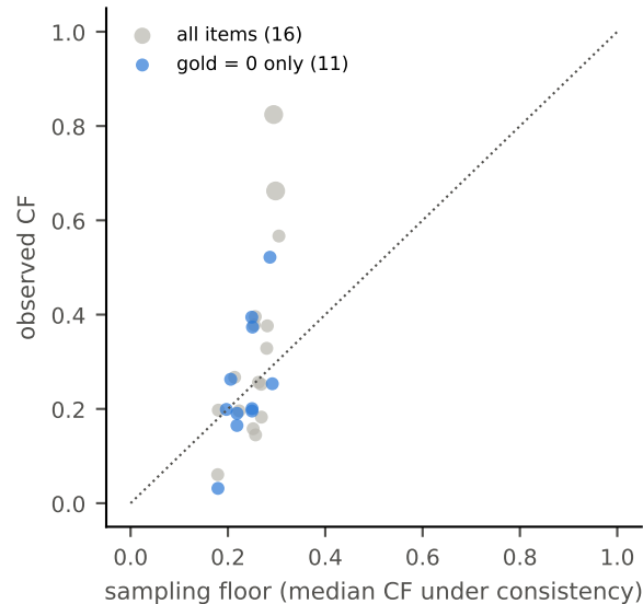
(a) tetrahedral covers: CF vs floor (large dots: BH-significant)
