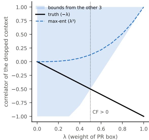
(a) CHSH: truth leaves the bounds iff CF > 0
