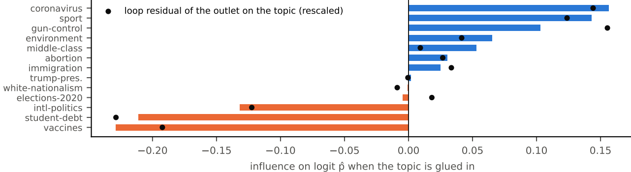
(a) Loop content: each topic's pull on breitbart \times gender (blue: gluing it in raises \hat{p} )
