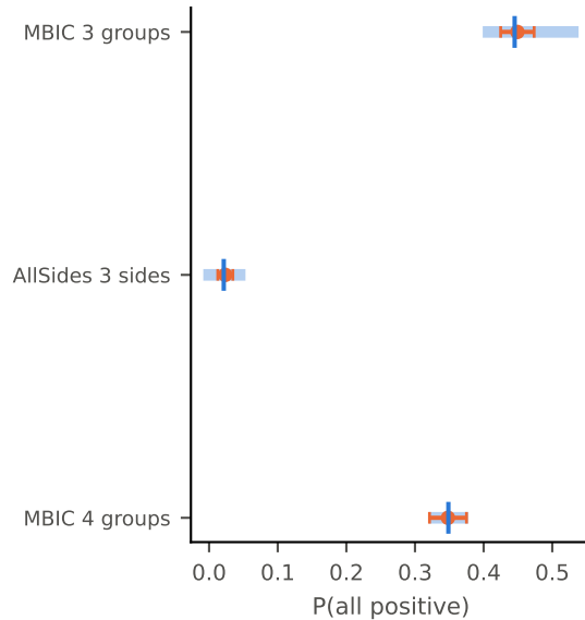
(c) outcome: [F] band, [T] tick, [I] dot
