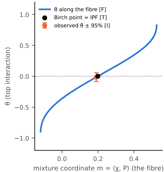
(a) MBIC 4 groups: fibre, variety, data
