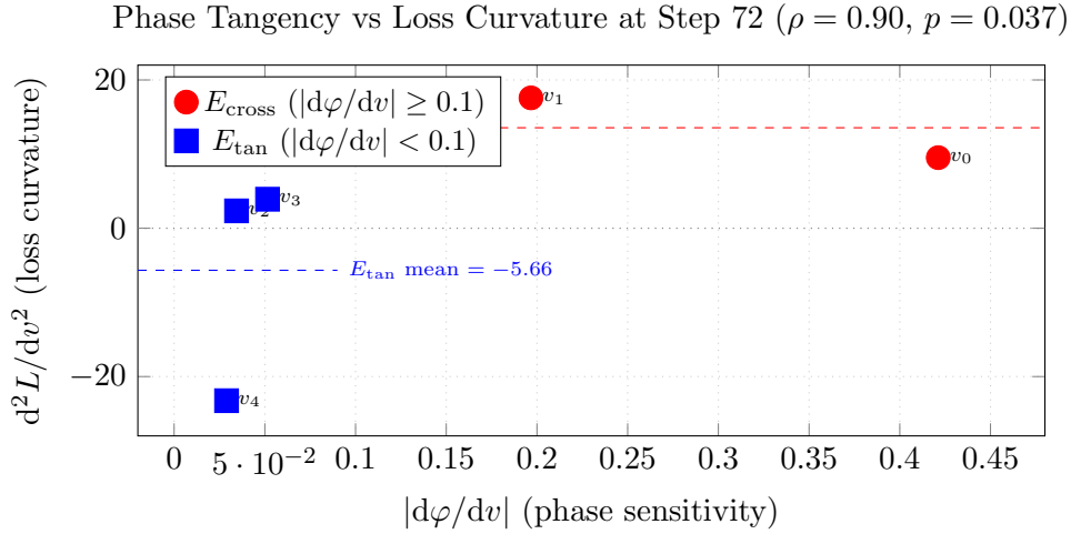
FIGURE 3. Phase sensitivity |\mathrm{d}\varphi/\mathrm{d}v| vs loss Hessian curvature \mathrm{d}^2L/\mathrm{d}v^2 for the five null eigenvectors at step 72 (Spearman \rho = 0.90 , p = 0.037 , n = 5 ). Red circles ( E_{\text{cross}} , v_0 and v_1 ): large phase sensitivity, positive loss curvature (loss-ascent directions). Blue squares ( E_{\text{tan}} , v_2, v_3, v_4 ): small phase sensitivity, negative or small loss curvature (loss-descent or flat directions). The phase-tangent directions at the codimension-2 crossing are precisely the loss-descent directions in the symplectic null space.
