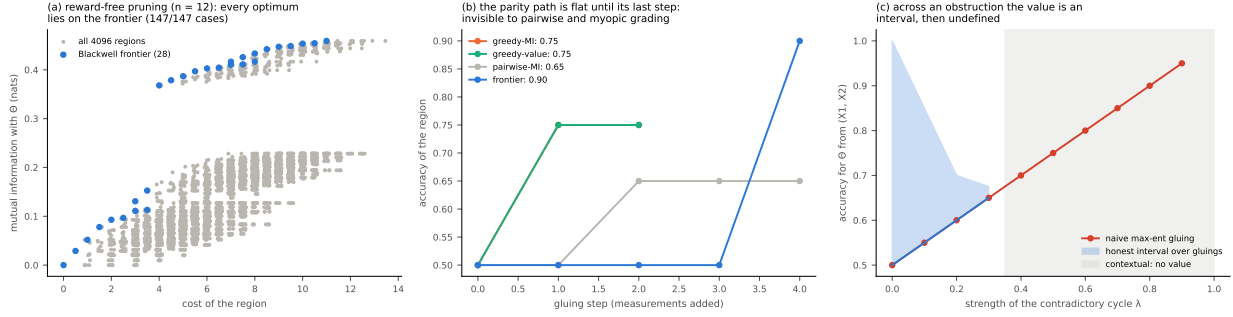
Figure 26: Blackwell-graded region search. (a) All 4096 regions ( n = 12 ) by cost and information, with the reward-free Blackwell frontier; every optimum lies on it. (b) Value along the growth path of the region each method picks under a budget of 4; the parity region is flat until its last gluing step. (c) Deciding \Theta from (X_1, X_2) across a contradictory cycle: naive glued value, honest interval over gluings, and the contextual range where no value exists.
