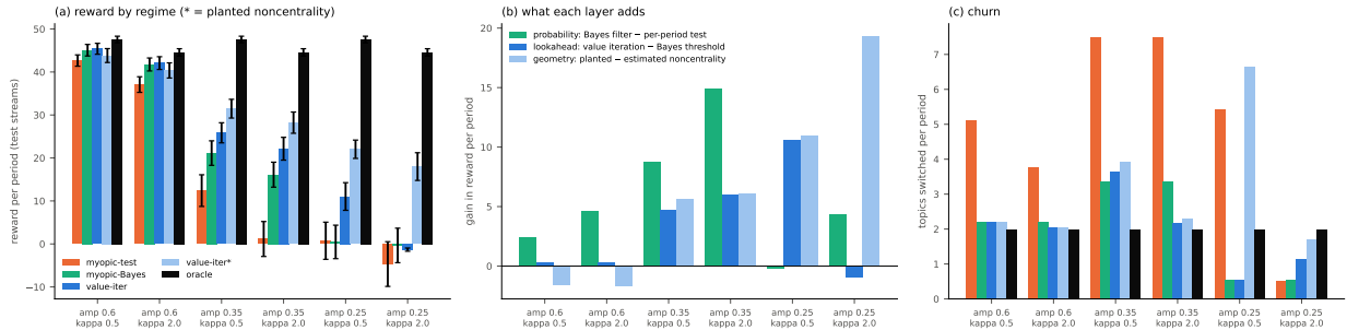
Figure 25: The reward loop. (a) Reward per period by regime (loop amplitude, switching cost \kappa ); * uses the planted noncentrality. (b) What each layer adds: probability (Bayes filter minus the per-period test), lookahead (value iteration minus the Bayes threshold), geometry (planted minus estimated noncentrality, for value iteration). (c) Topics switched per period.
