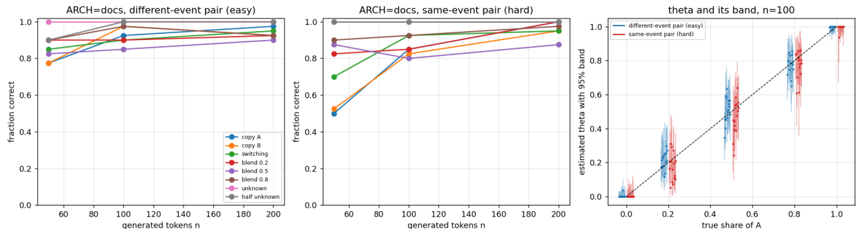
Figure 32: Context attribution. Fraction correct by case against the number of tokens for easy and hard pairs, and estimated share with its 95% band against the true share ( n = 100 ).
