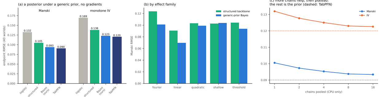
Figure 29: Generic-prior posterior on CausalIDView. (a) Endpoint RMSE over 40 worlds against logistic regression, the structured backbone and the published TabPFN. (b) Manski error by effect family. (c) Error against the number of chains pooled; dashed lines mark TabPFN.
