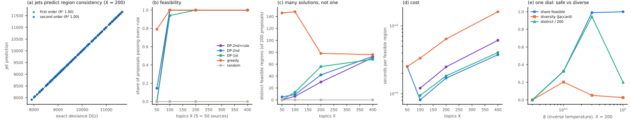
Figure 23: Dynamic programming on the gluing lattice. (a) Jet predictions of region consistency against the exact deviance ( X = 200 ). (b) Share of proposals passing every rule. (c) Distinct feasible regions among 200 proposals. (d) Seconds per feasible region. (e) The temperature dial at X = 200 : feasibility, diversity and distinct regions.
