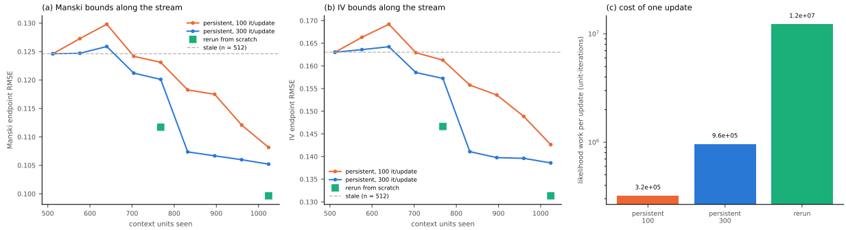
Figure 30: Persistent posteriors on a data stream (5 worlds, one per effect family). (a, b) Endpoint RMSE as context arrives: persistent chains updated with 100 or 300 iterations per batch, reruns from scratch at n = 768 and 1024, and the stale n = 512 posterior. (c) Likelihood work per update (log scale).
