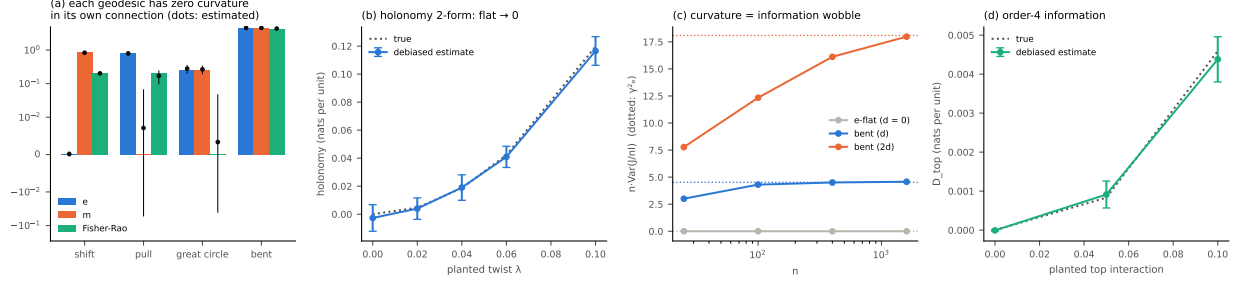
Figure 18: Planted checks for second-order information geometry. (a) Exact curvature of four planted paths in the e , m and Fisher–Rao connections (bars) and the bias-corrected estimates from counts (dots, \pm sd); each geodesic is flat in its own connection. (b) Holonomy information on a planted twist: debiased estimate against truth. (c) n \text{Var}(J/nI) against n ; dotted lines are \gamma_e^2 . (d) Order-4 information against a planted top interaction.
