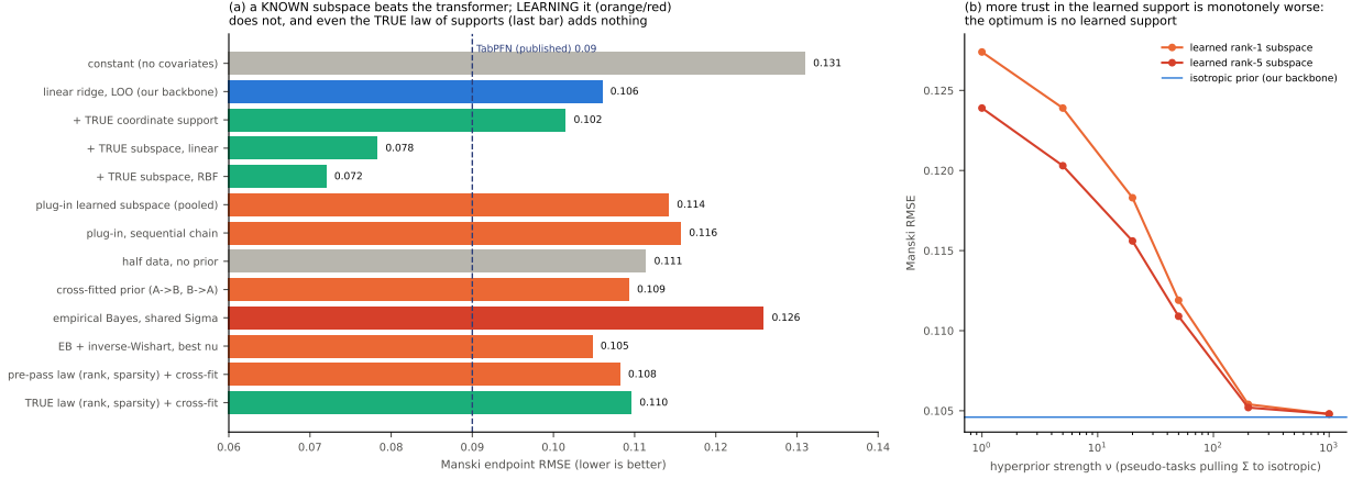
Figure 28: Support-guided priors on CausalIDView (Manski view). (a) A known subspace (green) beats the published transformer; every way of learning it inside one world (orange, red) does not beat no support, and even the true law of supports (rank and sparsity, last bar) adds nothing. (b) Empirical Bayes with an inverse-Wishart hyperprior: the more weight the learned subspace gets, the worse the fit.
