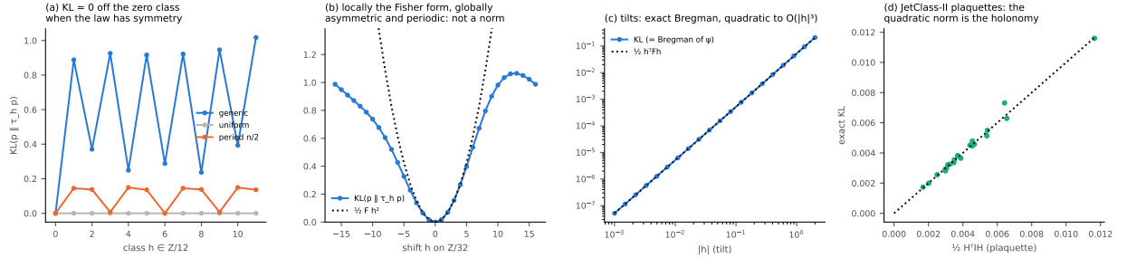
Figure 20: Statistical holonomy and the class. (a) KL by class on \mathbb{Z}/12 : zero off the zero class for symmetric laws. (b) Shifts on \mathbb{Z}/32 : locally \frac{1}{2}Fh^2 , globally asymmetric and periodic. (c) Tilts: KL equals the Bregman divergence of \psi and is quadratic to O(|h|^3) . (d) JetClass-II plaquettes: exact KL against \frac{1}{2}H^\top IH .
