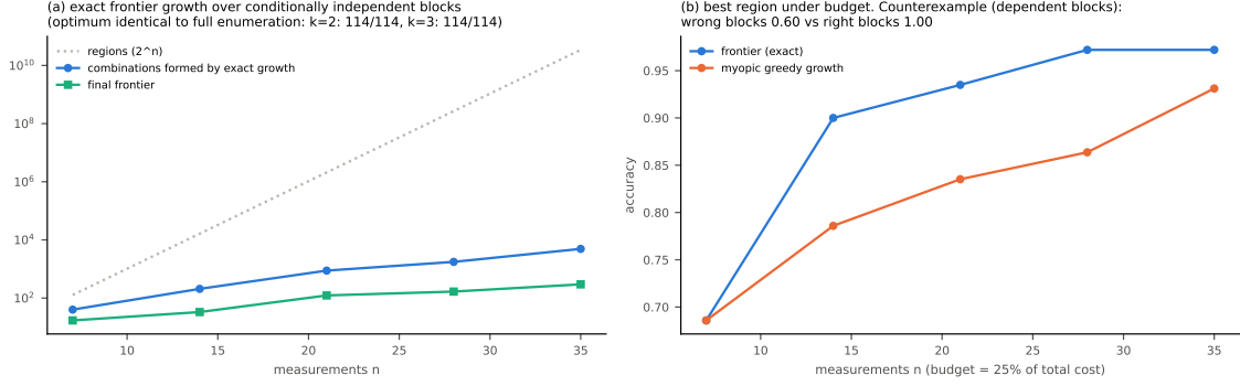
Figure 27: Exact frontier growth. (a) Combinations formed by block growth and final frontier size, against the 2^n regions of enumeration; the optimum matched enumeration in every check for k = 2 and k = 3 . (b) Best accuracy under a budget, exact frontier against myopic greedy growth; the title gives the counterexample with dependent blocks.
