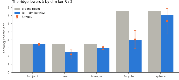
Figure 21: The flat ridge of margin data lowers the learning coefficient by \dim \ker R/2 : d/2 , the predicted \lambda , and the WBIC estimate ( \pm 1.96 se) on five covers.
