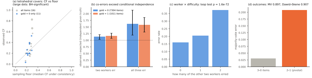
Figure 16: Crowdsourced entity resolution. (a) CF of each tetrahedral worker cover against its sampling floor, for all items and for gold-negative items; large dots are Benjamini–Hochberg significant. (b) Co-errors observed over expected under independence given the truth (item bootstrap, 95%). (c) Error rate by how many of the other two workers erred. (d) Majority-vote error on unanimous and pivotal items.
