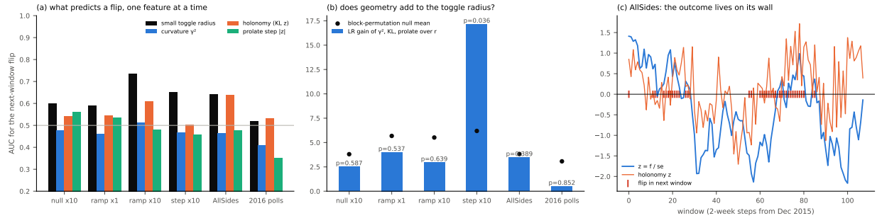
Figure 22: Flip prediction. (a) AUC of each feature for the next-window flip. (b) Likelihood-ratio gain of curvature, holonomy and the prolate test over the toggle radius, against the block-permutation null mean. (c) AllSides: f/se , the holonomy z , and windows followed by a flip.
