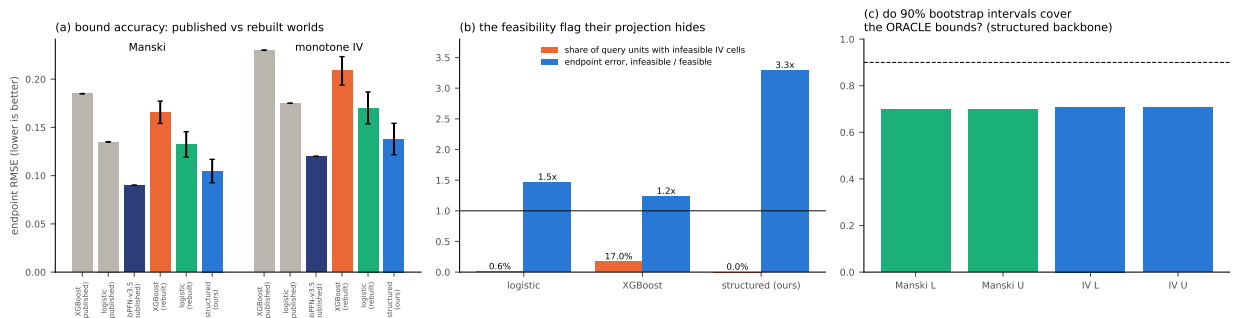
Figure 31: CausalIDView partial identification. (a) Endpoint RMSE, published values (Jung et al.) against the rebuilt worlds, for the Manski and monotone-IV views. (b) Share of query units with infeasible estimated IV cells, and their endpoint error relative to feasible units (for the structured backbone the ratio rests on a single unit). (c) Coverage of the oracle endpoints by 90% context-bootstrap intervals (structured backbone; the IRLS backbone gives 81–82%).
