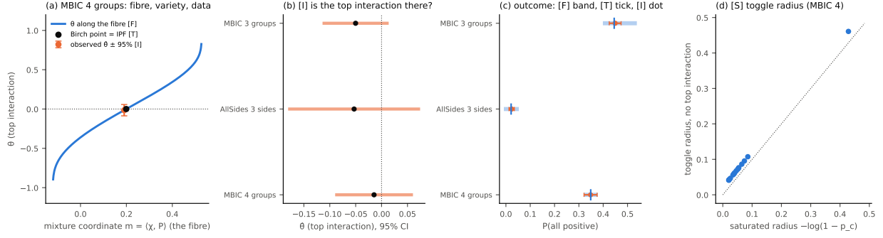
Figure 11: The four components. (a) MBIC four groups: \theta along the fibre [F] (mixture coordinate on the horizontal axis); the Birch point, equal to IPF [T]; the observed \hat{\theta} with its 95% interval [I]. (b) \hat{\theta} with 95% intervals for the three tables with full joints. (c) One outcome, P(\text{all positive}) , through the components: [F] bounds (band), [F]+[T] maximum-entropy point (tick), [I] observed (dot with interval). (d) [S] Exact toggle radius of each cell in the no-top-interaction model against the saturated radius (MBIC four groups).
