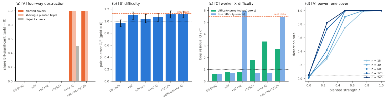
Figure 17: Planted positives and nulls on the real crowdsourcing design. (a) [A] Share of tetrahedral covers flagged after Benjamini–Hochberg: planted, sharing a planted triple, and disjoint. (b) [B] Pair co-error ratio (gold 0), with the real value dashed. (c) [C] Loop residual of the worker \times difficulty model with the proxy difficulty and with the true difficulty; real value dashed. (d) [A] Power for one cover by items per triple and planted strength; the dotted line is the nominal 5%.
