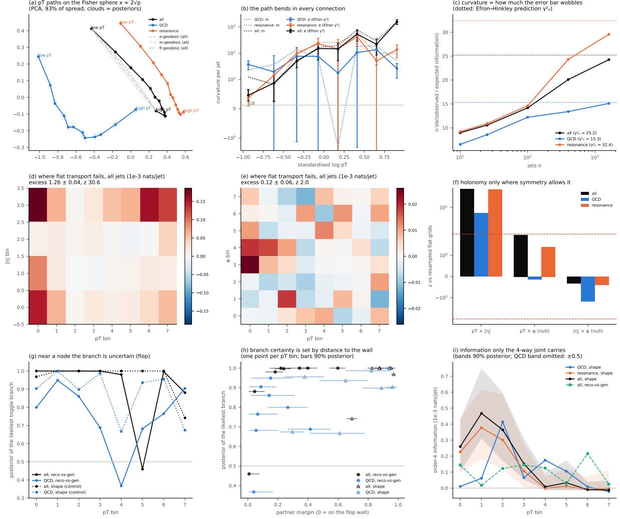
Figure 19: Second-order information geometry on JetClass-II. (a) The p_T paths as points 2\sqrt{p} on the Fisher sphere (first two principal components), with posterior clouds and the e -, m - and FR-geodesics between the end bins. (b) Debiased curvature along p_T : e (Efron \gamma^2 , with sd) and m (dotted). (c) Error-bar wobble n \text{Var}(J/nI) against n , approaching \gamma_e^2 (dotted). (d, e) Where flat transport fails: excess information per grid cell on p_T \times |\eta| and on the null grid p_T \times \varphi . (f) Holonomy z -scores against resampled flat grids; the dashed lines are \pm 2 . (g) Posterior of the likeliest toggle branch by p_T , near the node (reco-versus-gen) and far from it (shape). (h) Branch certainty against the partner margin, one point per table and p_T bin. (i) Order-4 information by p_T .
