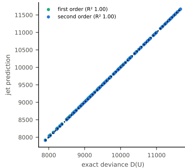
(a) jets predict region consistency ( X = 200 )
