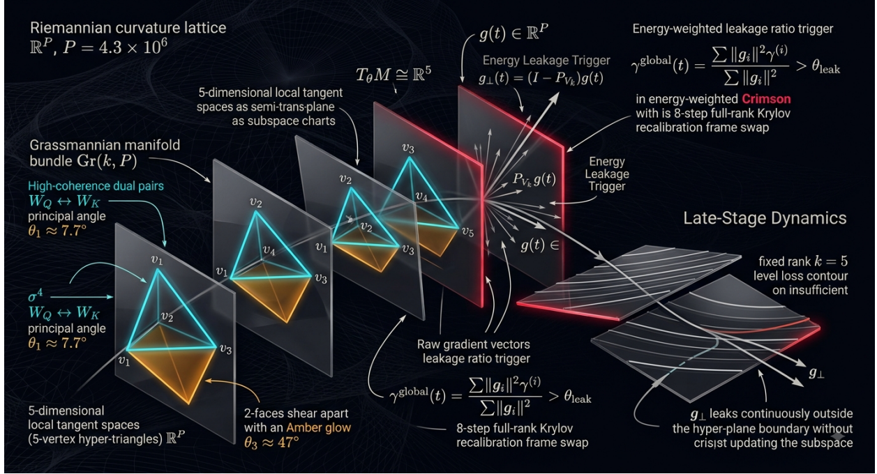
FIGURE 9. The controller. Per-block motion occupies low-dimensional charts on \text{Gr}(k, P) ; the energy-weighted leakage ratio \gamma^{\text{global}} = \sum_i \|g_i\|^2 \gamma^{(i)} / \sum_i \|g_i\|^2 measures how much of a fresh gradient falls outside the current frame, and crossing \theta_{\text{leak}} triggers a short full-rank window in which every frame is re-estimated. At P = 4.3 \times 10^6 the leakage never falls below threshold and the frame is continuously outrun, which is the failure mode drawn at right.
