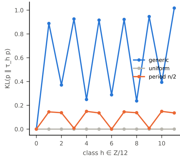
(a) KL = 0 off the zero class when the law has symmetry
