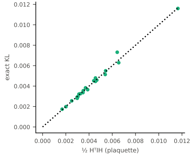
(d) JetClass-II plaquettes: the quadratic norm is the holonomy
