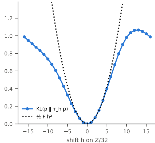
(b) locally the Fisher form, globally asymmetric and periodic: not a norm
