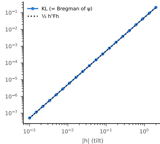
(c) tilts: exact Bregman, quadratic to O(|h|^3)
