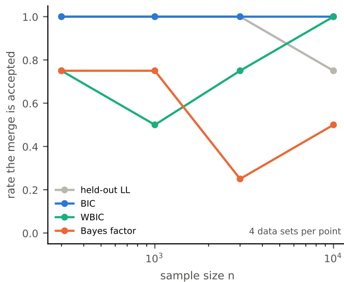
(b) spurious split (truth K_0=2 , candidate K=3 )
