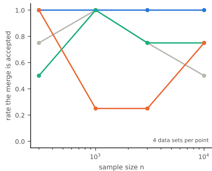
(c) weak real split (truth K_0=3 , two symbols close)
