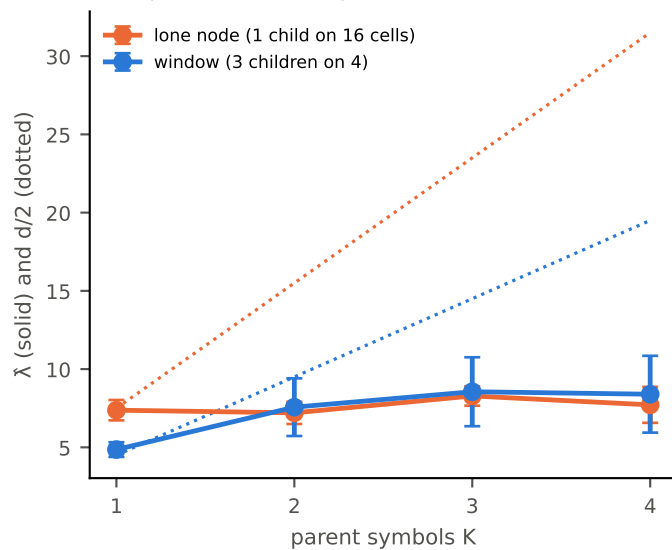
(a) \lambda plateaus: extra symbols cost \ll d/2
