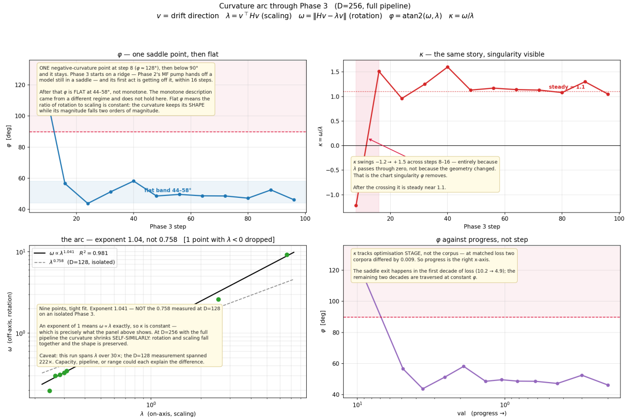
FIGURE 10. The curvature arc through Phase 3 of the full pipeline at D = 256 . \lambda = v^\top H v is the on-axis response of the drift to curvature, \omega = \|Hv - \lambda v\| the off-axis response, \varphi = \text{atan2}(\omega, \lambda) and \kappa = \omega/\lambda . Top left: one negative-curvature point at step 8 ( \varphi \approx 128^\circ ), then \varphi flat at 44\text{--}58^\circ . Top right: the same story with the chart singularity visible — \kappa swings -1.2 \rightarrow +1.5 purely because \lambda crosses zero. Bottom left: the arc, exponent 1.041 at R^2 = 0.981 , with the 0.758 of §54 shown dashed for contrast. Bottom right: \varphi against progress rather than step.
