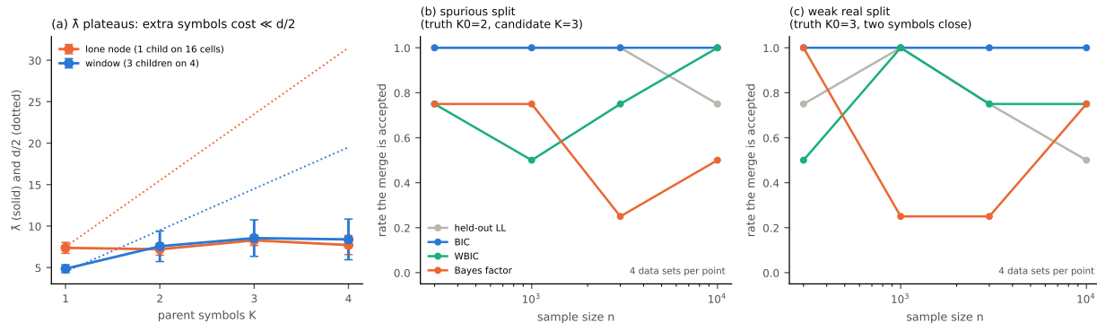
Figure 15: Split-merge and the learning coefficient. (a) \hat{\lambda} (solid, 95% Monte-Carlo intervals) against d/2 (dotted) by the number of parent symbols, for a lone node (one child on 16 cells) and an identifying window (three children on 4); true K_0 = 2 . (b, c) How often each criterion accepts the merge back to K_0 for a spurious split (b) and a weak real split (c), over n (4 data sets per point).
