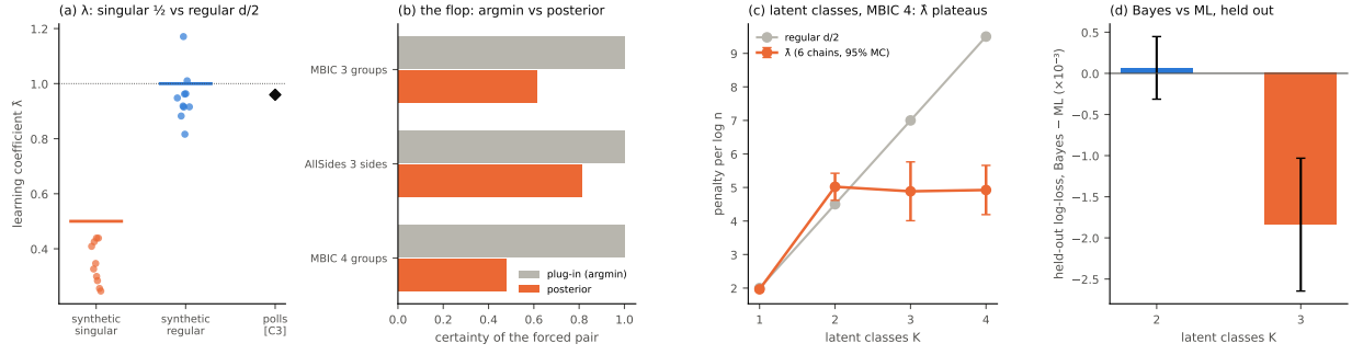
Figure 14: Singular statistics. (a) \hat{\lambda} on synthetic singular and regular truths (bars: theory) and on the polls mixture. (b) Certainty of the support toggle's forced pair: plug-in argmin (implicitly 1) against the Dirichlet posterior. (c) Latent-class models on MBIC four groups: the regular penalty d/2 against \hat{\lambda} (95% Monte-Carlo intervals). \hat{\lambda} plateaus near 5 while d/2 keeps growing. (d) Held-out log-loss per sentence of the Bayes predictive minus ML plug-in (40 random halves; 95% intervals).
