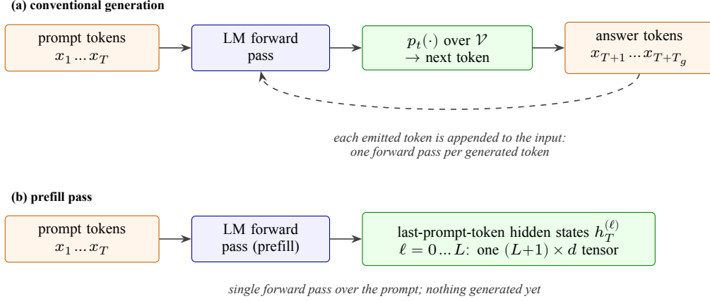
Figure 1: Token flow in the two forward-pass regimes. (a) Conventional generation: one forward pass per generated token; the emitted token is appended to the input and fed back, so the answer is produced autoregressively. (b) Prefill pass: a single forward pass over the prompt alone; nothing is generated yet, and the last-prompt-token hidden state h_T^{(\ell)} is available at every layer \ell . The dimensions used throughout ( L=28 layers, d=2048 , a 29 \times 2048 tensor per question) are specific to Qwen3-1.7B; the other subject models differ in both depth and width.
