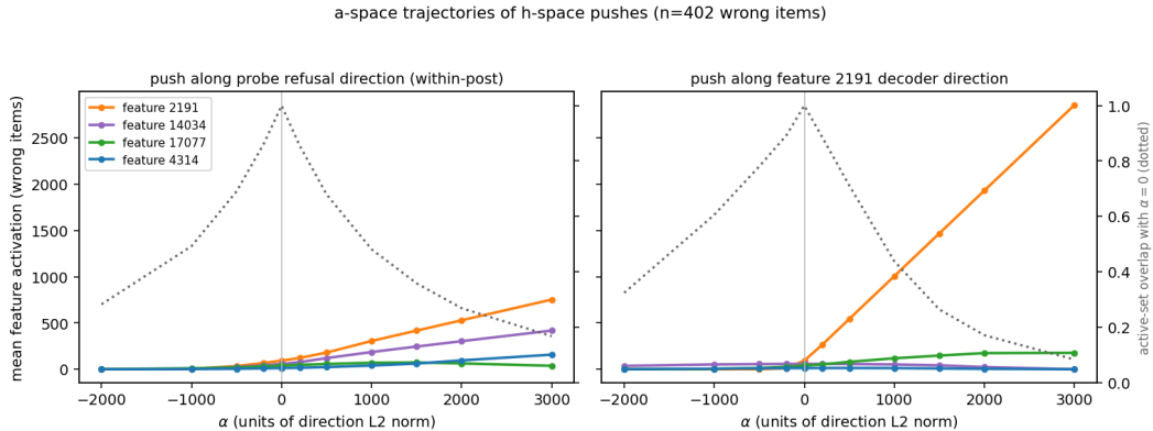
Figure 12: a-space trajectories of h-space pushes ( n = 402 wrong items, pre-norm residuals). Solid lines: mean activation of four ensemble features as the state is pushed along the Section 6.2 refusal direction (left) or feature 2191’s decoder direction (right); dotted: mean overlap (Jaccard) of the active feature set with the unperturbed code. The probe push recruits the register broadly; the 2191 push concentrates on the opener and crowds out the hedge.
