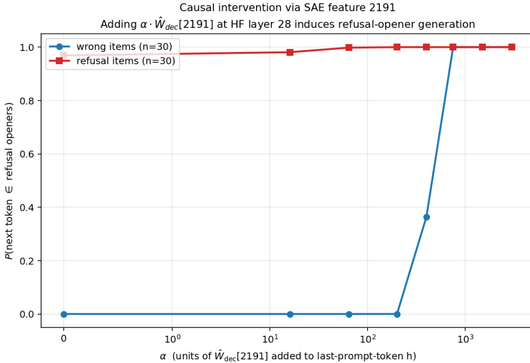
Figure 13: Causal dose-response of SAE feature 2191. On 30 ConfabQA wrong items (blue), adding \alpha \cdot \hat{W}_{\text{dec}}[2191] to the last-prompt-token post-block-27 residual induces a sharp transition between \alpha = 200 and \alpha = 750 from no refusal-opener probability to 100% of next-token mass on refusal openers (and 30/30 argmax flips). The 30 ConfabQA refusal items (red) are already saturated at \alpha = 0 .
