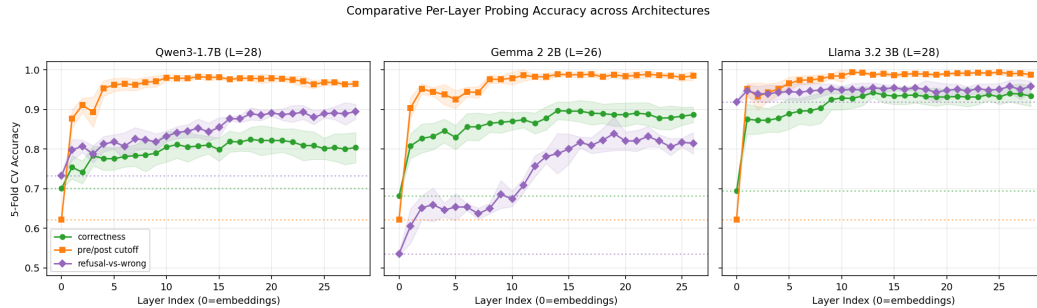
Figure 15: Comparative probing accuracy curves across Qwen3-1.7B, Gemma 2 2B, and Llama 3.2 3B.
