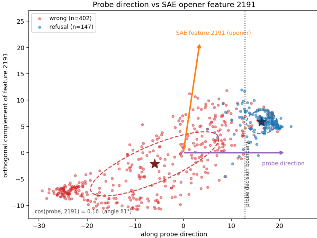
Figure 14: The plane spanned by the probe refusal direction and SAE feature 2191’s decoder vector (refusal+wrong states in the probes’ representation, n = 549 ; stars: class centroids; dashed: per-class 1\sigma covariance ellipses). The two arrows are 81^\circ apart (cosine 0.16), yet the probe axis carries the class split and its decision boundary (dotted) is exact in this plane: a nearly probe-orthogonal output knob and a broad discriminative mixture share one causal channel.
