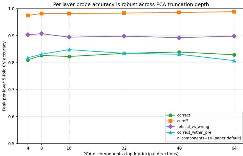
Figure 17: Peak per-layer probe accuracy as a function of PCA n_{\text{components}} , for each of the main probe targets. The paper default ( n = 16 ) is marked. All targets are stable across the sweep within a \leq 5\% band, and several peak at n \neq 16 , meaning the paper default is conservative rather than tuned.
