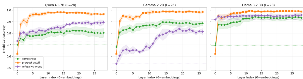
Figure 12: Comparative probing accuracy curves across Qwen3-1.7B, Gemma 2 2B, and Llama 3.2 3B.
