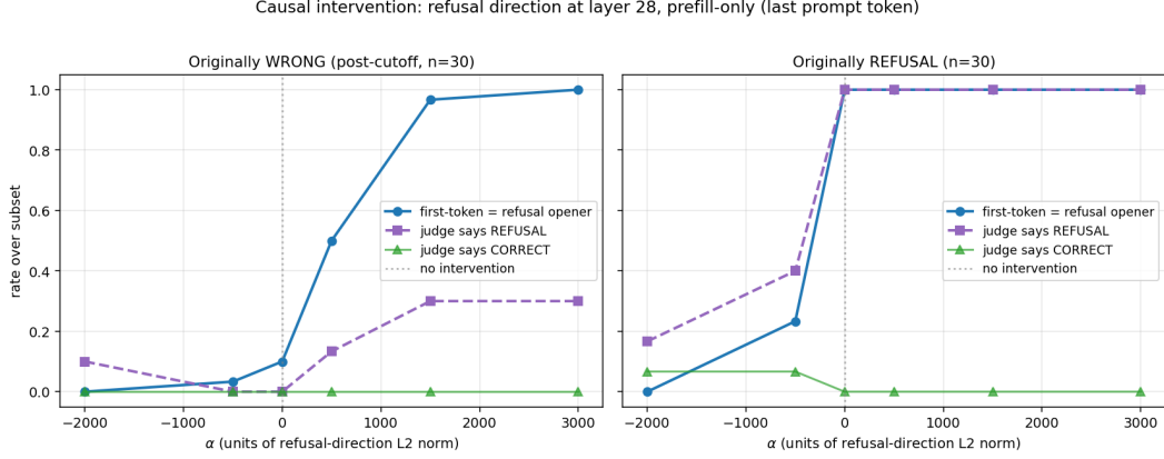
Figure 9: Causal intervention: rate over each subset as a function of \alpha . Solid blue: fraction of generations whose first generated token matches a refusal opener ( { as, As, as, 作为, ... } ). Dashed purple: fraction whose full judge label is REFUSAL. Light green: fraction labeled CORRECT (drops at high |\alpha| on the refusal subset: intervention can also break originally correct refusals into confabulations). The first-token measure changes monotonically and saturates near \alpha = \pm 1500 ; the full-judge measure changes more slowly because of autoregressive continuation dynamics.
