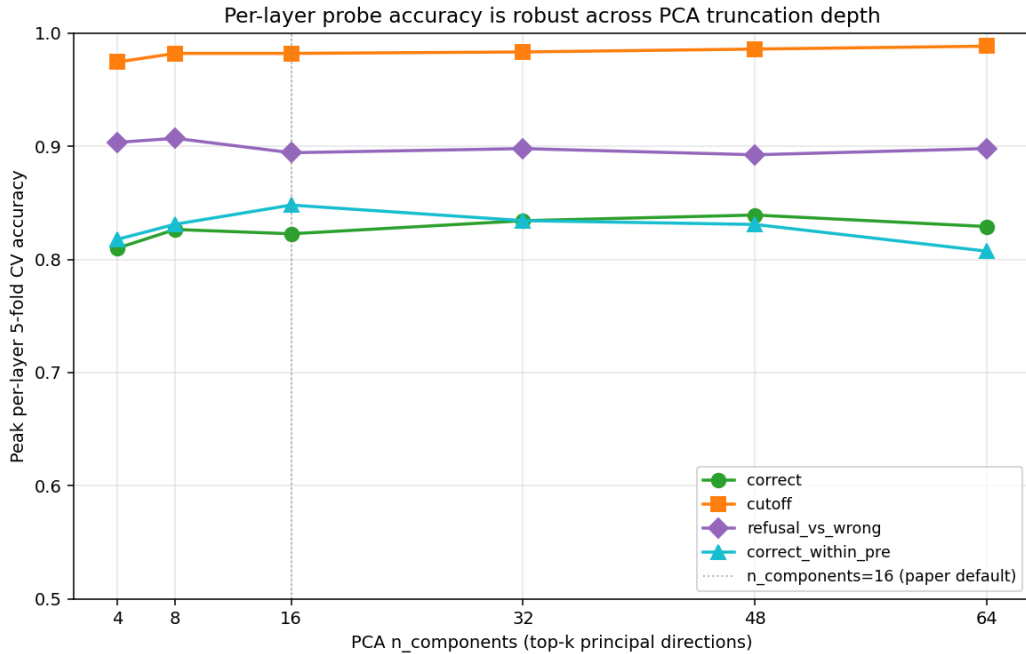
Figure 14: Peak per-layer probe accuracy as a function of PCA n_{\text{components}} for each of the main probe targets. The paper default ( n = 16 ) is marked. All targets are stable across the sweep within a \leq 5 pp band, and several peak at n \neq 16 , meaning the paper default is conservative rather than tuned.
