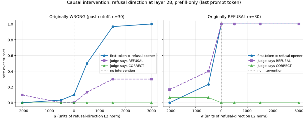
Figure 9: Causal intervention: rate over each subset as a function of \alpha . Solid blue: fraction of generations whose first generated token matches a refusal opener ( { as, As, as, 作为, ... } ). Dashed purple: fraction whose full judge label is REFUSAL. Light green: fraction labeled CORRECT (drops at high |\alpha| on the refusal subset: intervention can also break originally correct refusals into confabulations). The first-token measure changes monotonically and saturates near \alpha = \pm 1500 ; the full-judge measure changes more slowly because of autoregressive continuation dynamics.
